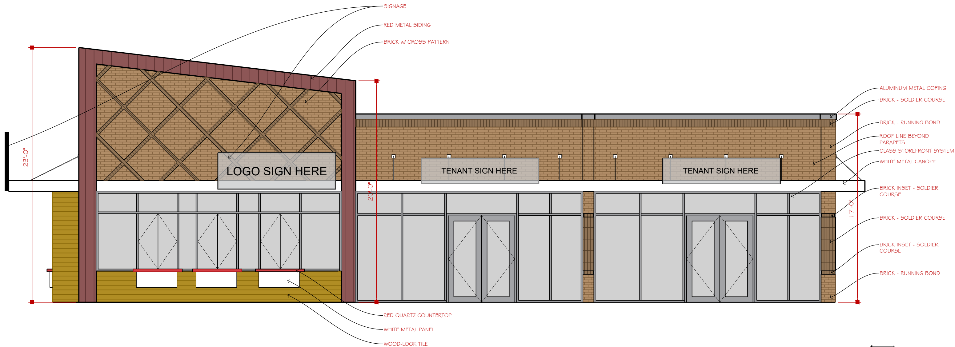
southeast elevation 1 1/8" = 1' - 0"
