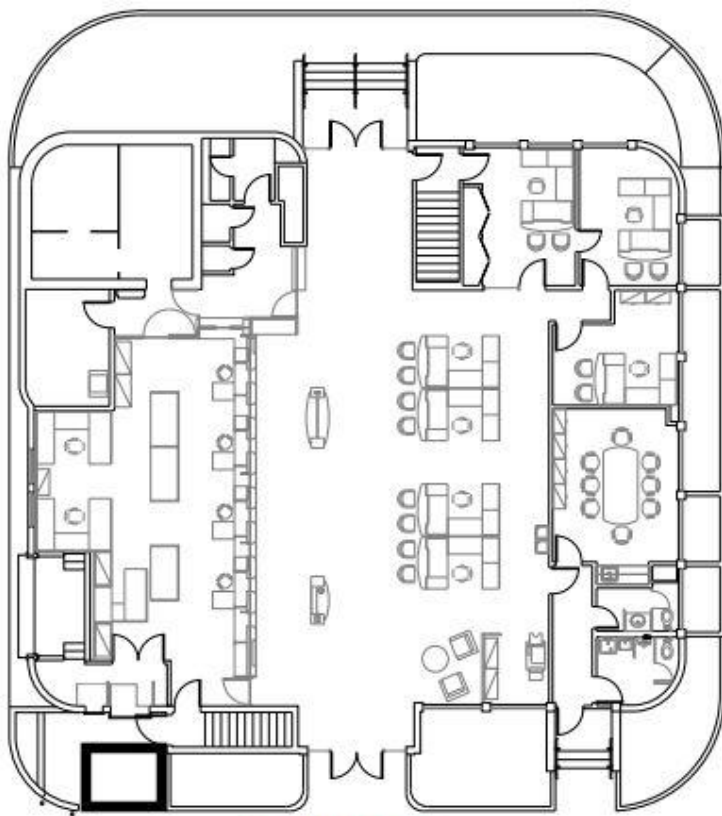
GROUND LEVEL
