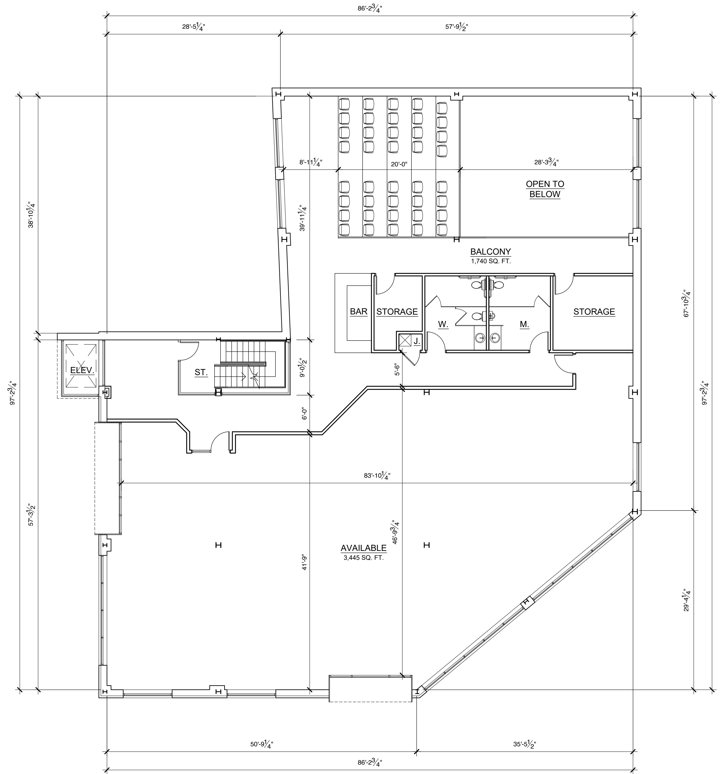
SECOND LEVEL PLAN SCALE: 1/8"=1'-0"
