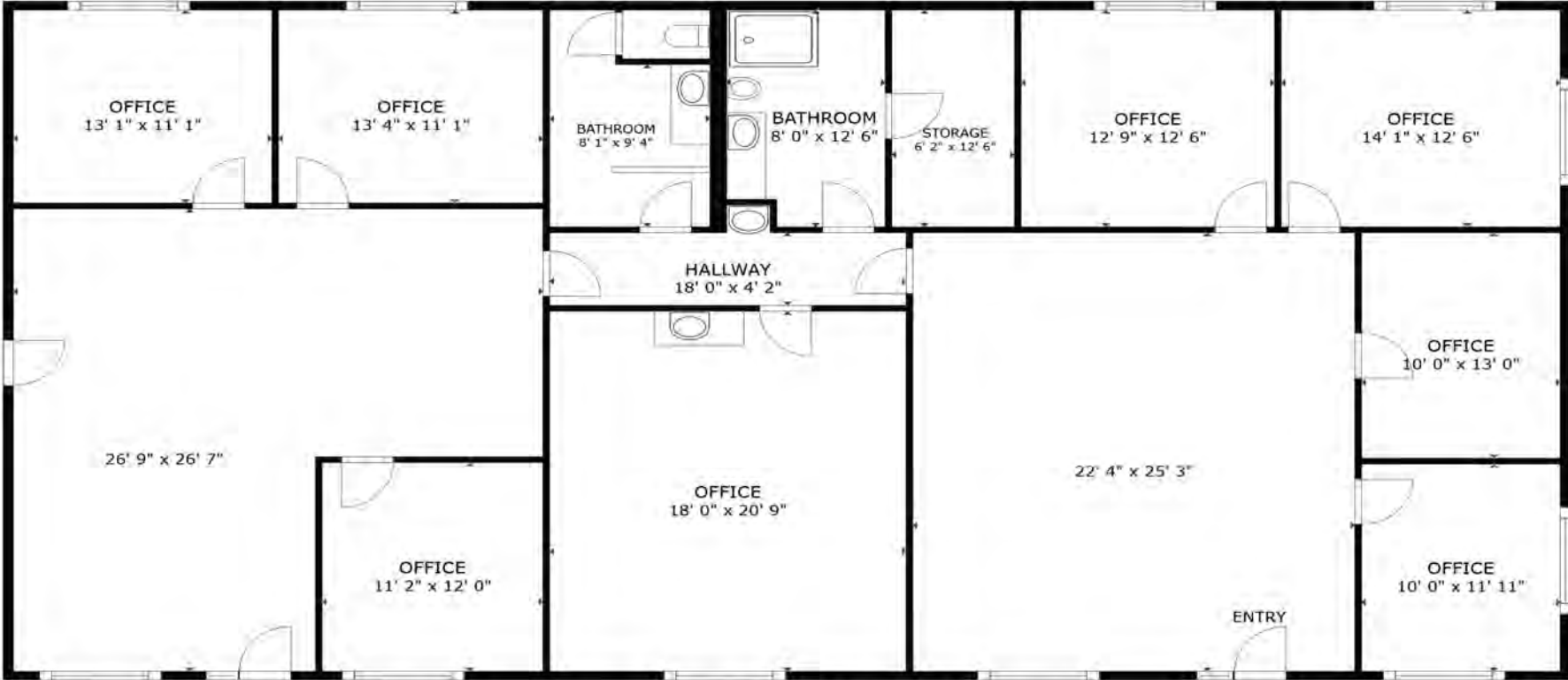
FLOOR PLAN
