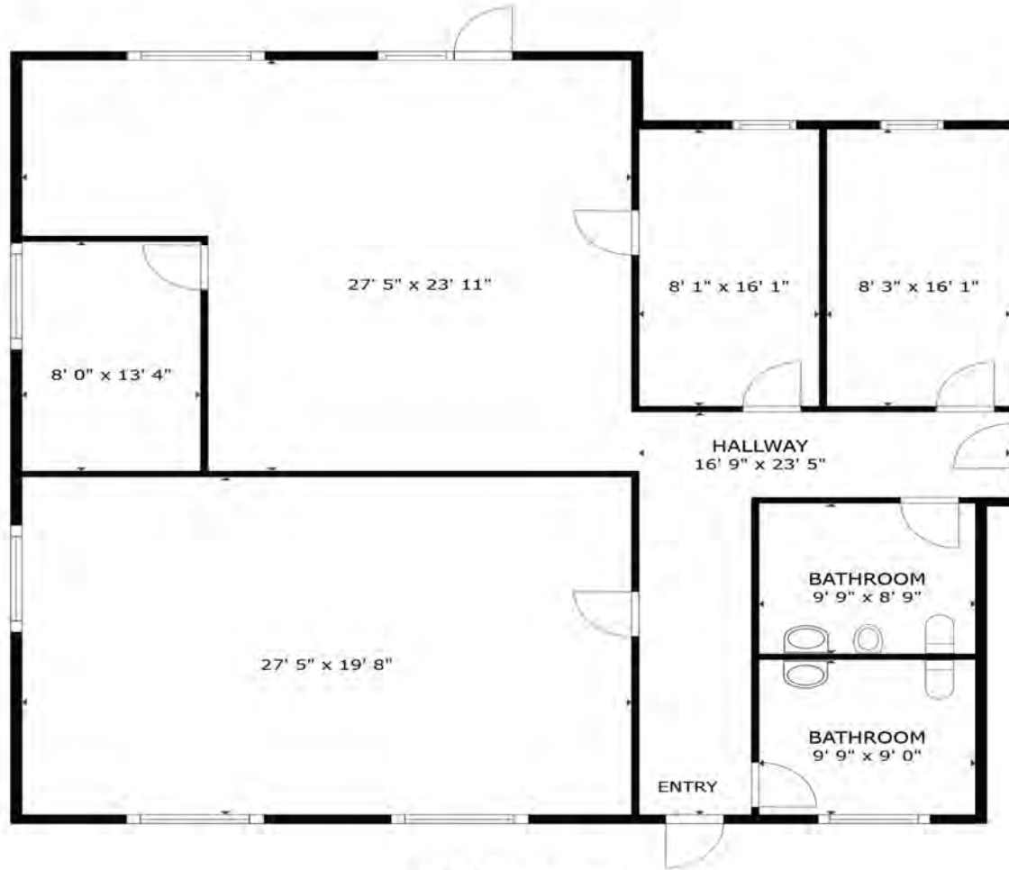
FLOOR PLAN
