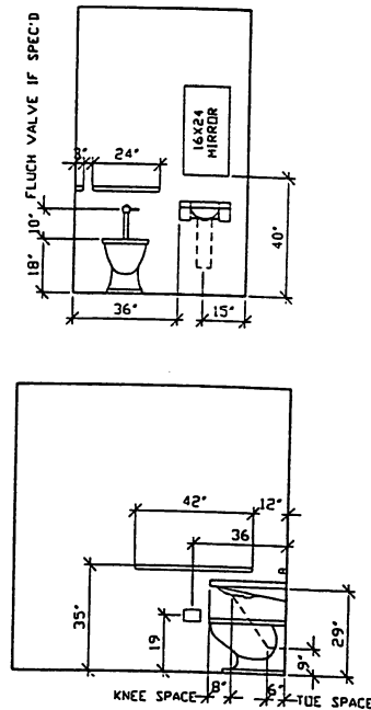
ELEVATIONS TYPICAL HANDICAPPED DIMENSIONS NO SCALE
