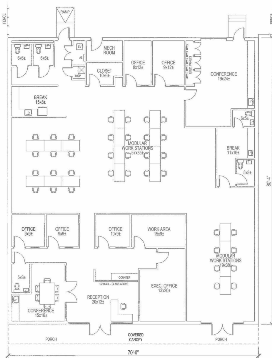
BUILDING PLAN - 5,630 S.F. (6,008 S.F. WITH FRONT COVERED CANOPY) 411 N. MAIN STREET EULESS, TEXAS Revised: 9/5/24
