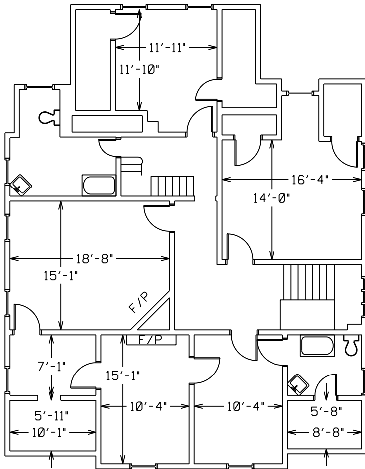
SECOND FLOOR
