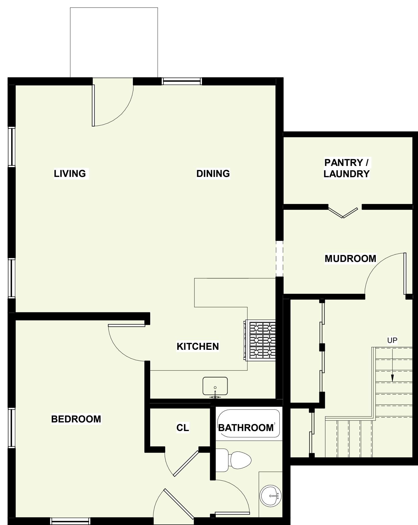
1 HOUSE FIRST FLOOR A-103 1/4" = 1'-0"
