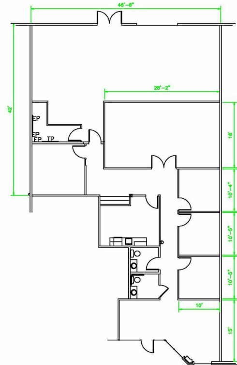
SPACE PLAN 1/16" = 1'-0"
