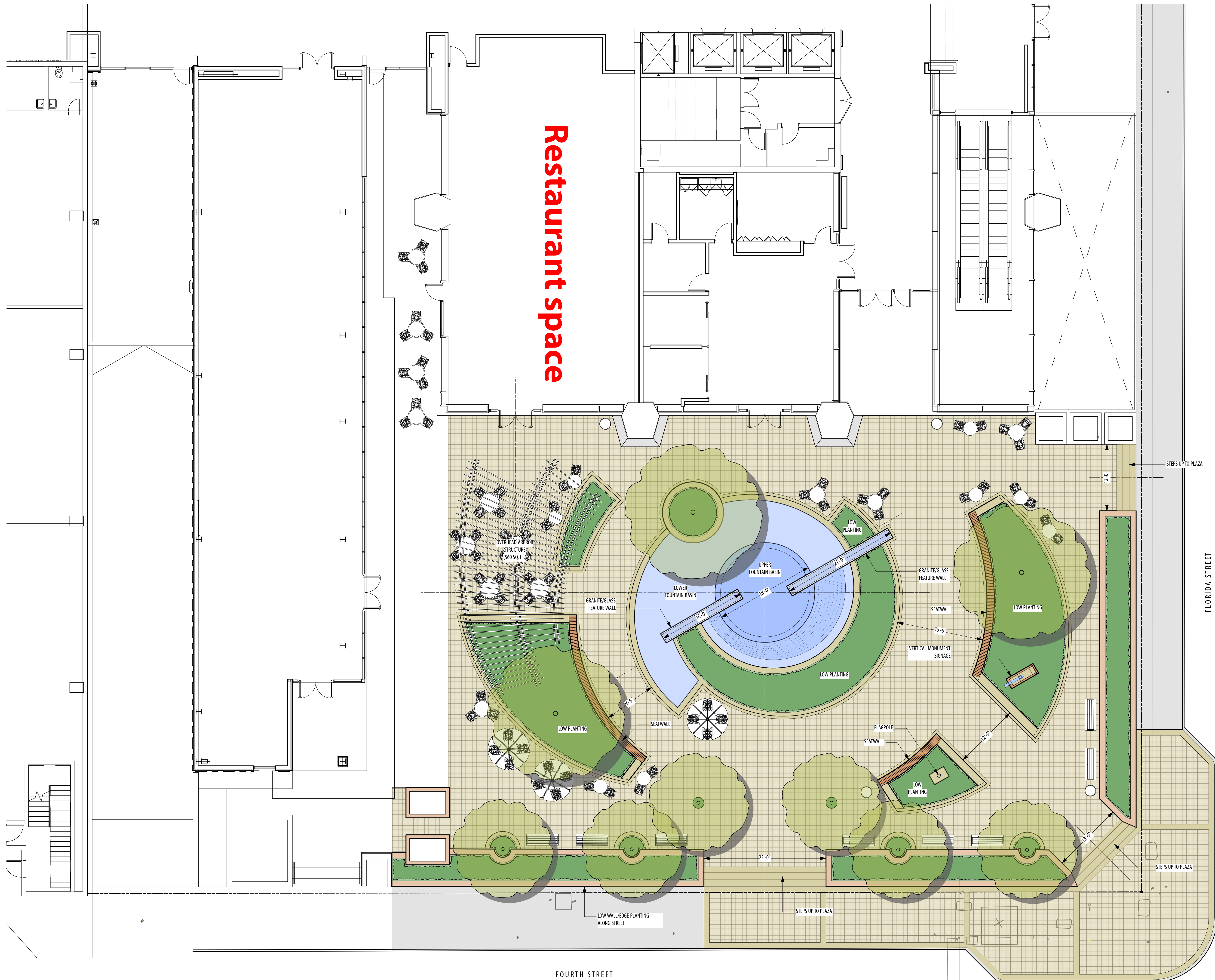
1 Schematic Design Plan - West Plaza L.01 Scale: 1/8" = 1'-0"
