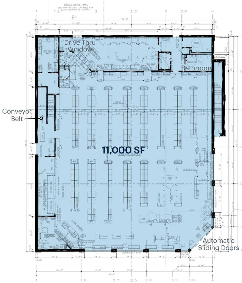
Ground Floor
