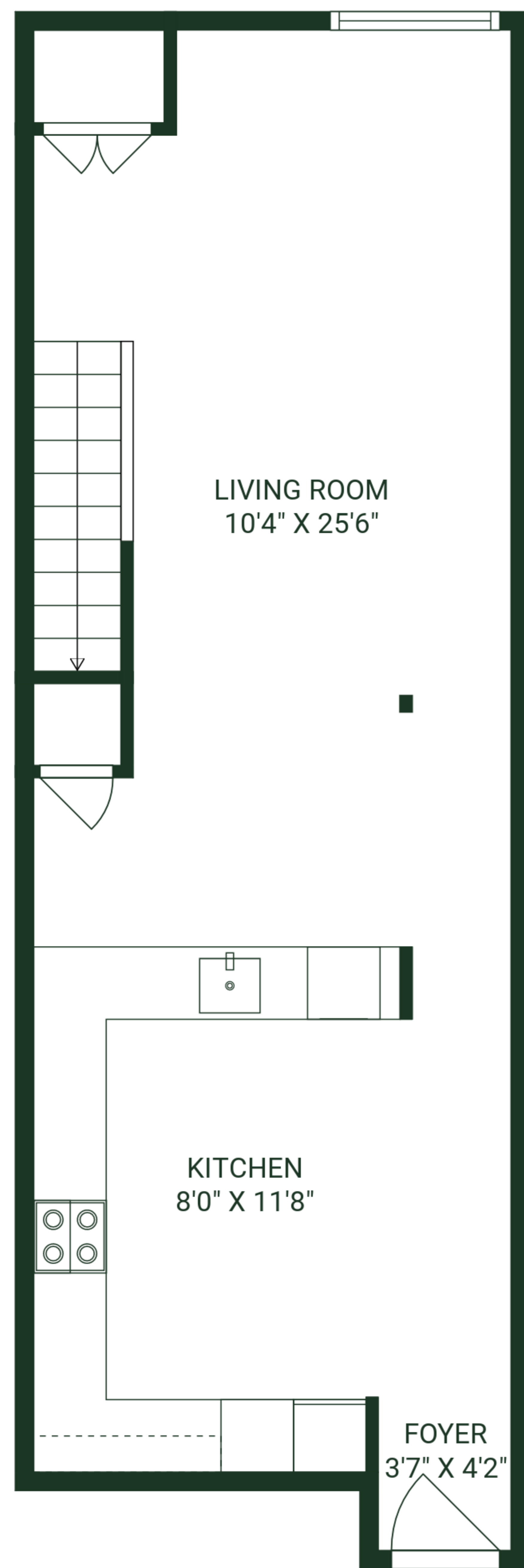
FLOOR 1
