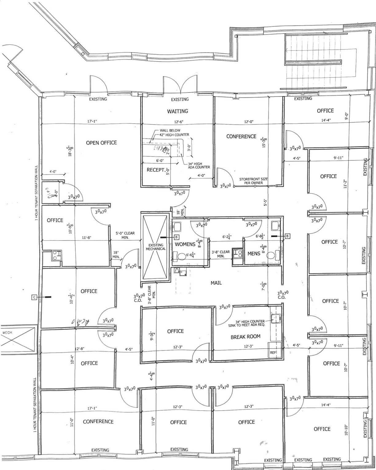
A FLOOR PLAN SCALE: 1/4" = 1'-0"
