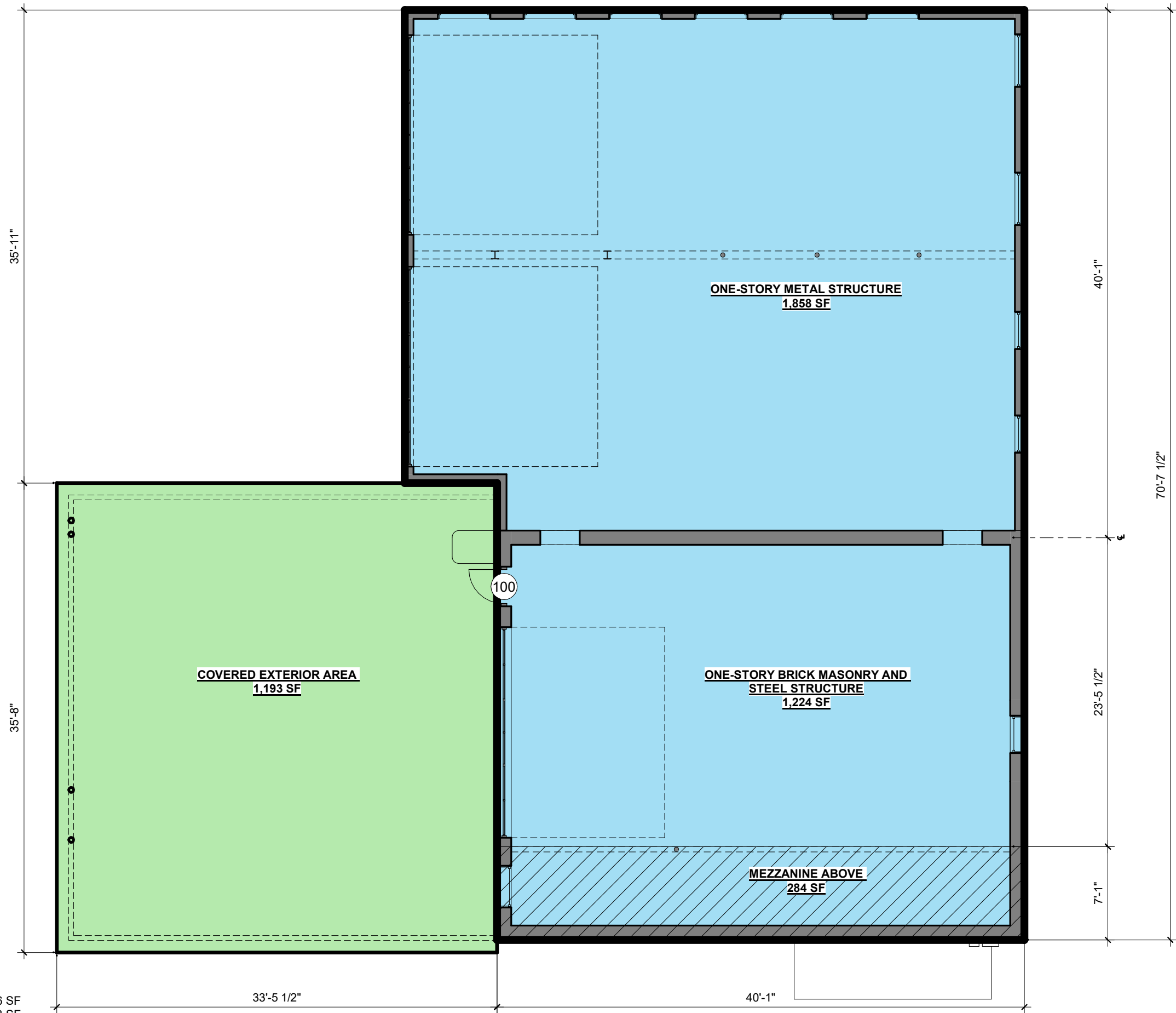
BUILDING D SQUARE FOOT DIAGRAM
