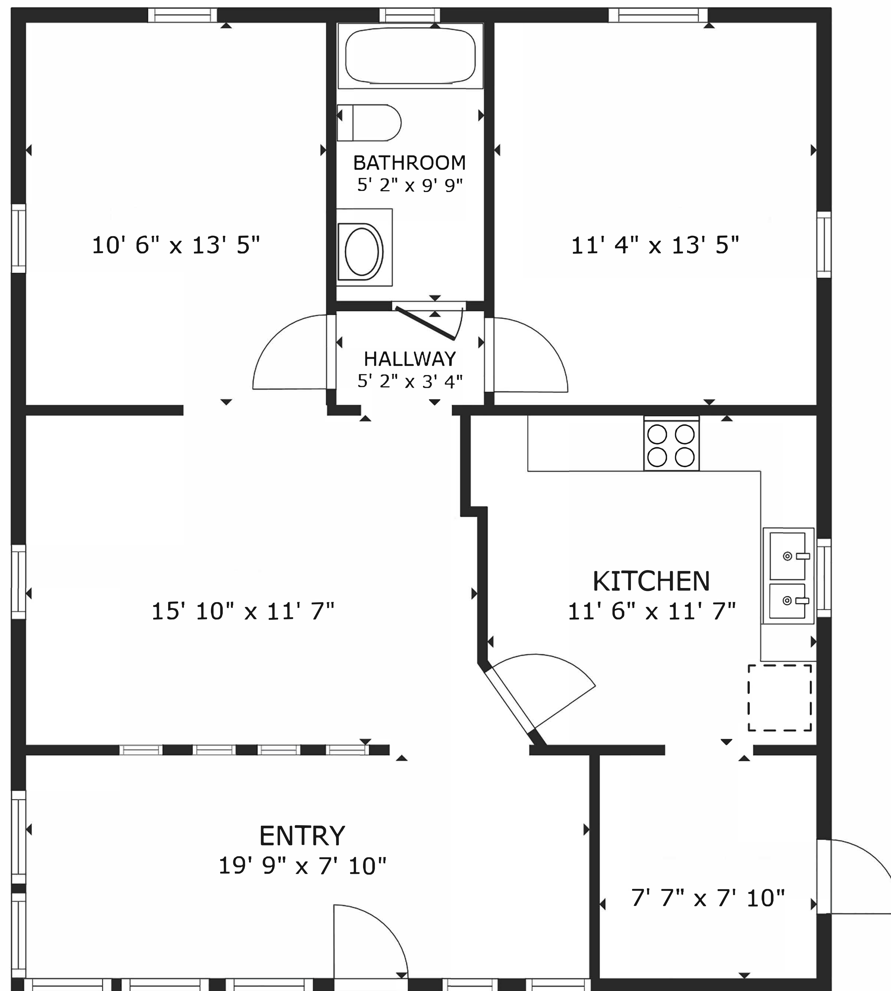
FLOOR PLAN
