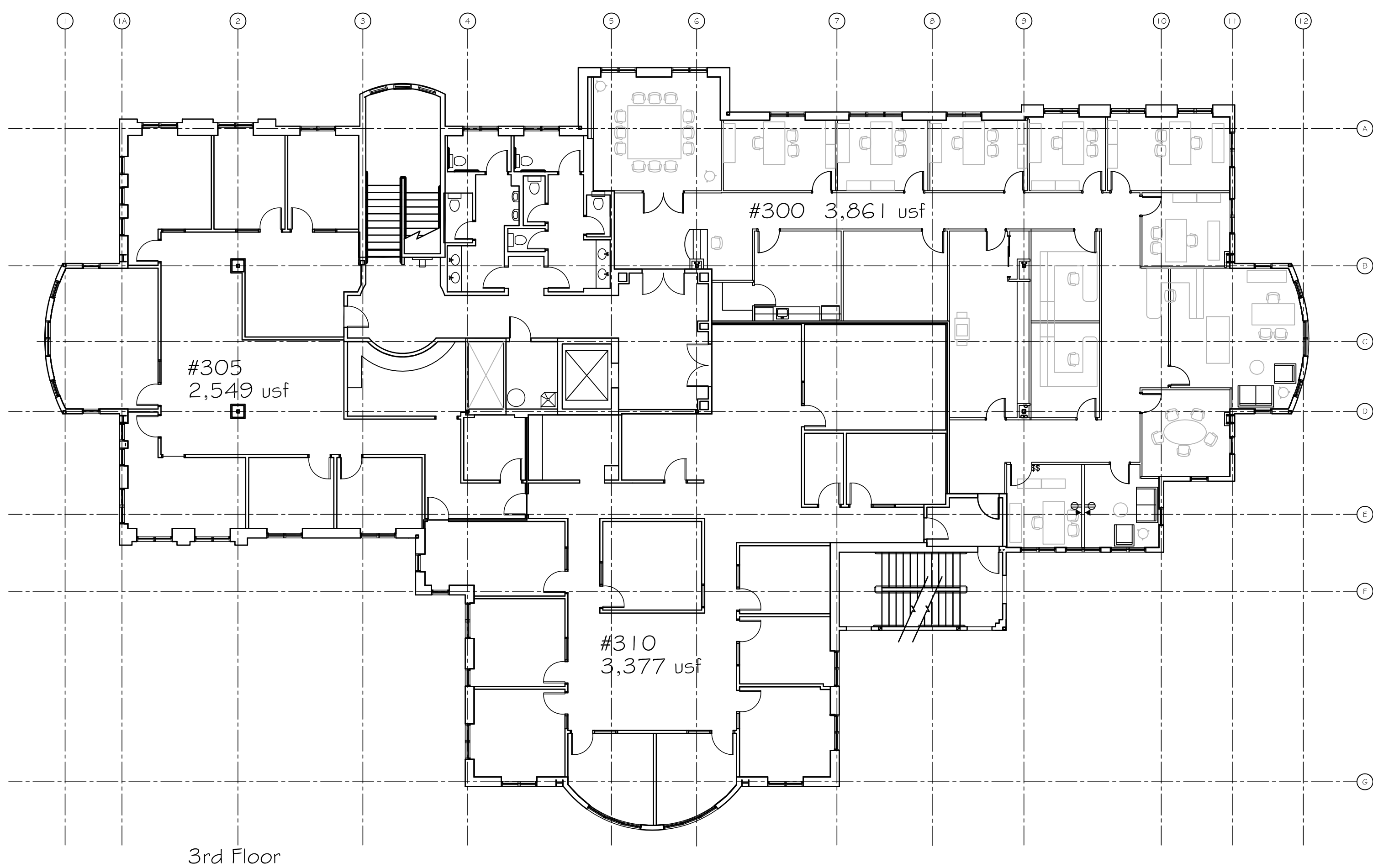
3rd Floor
