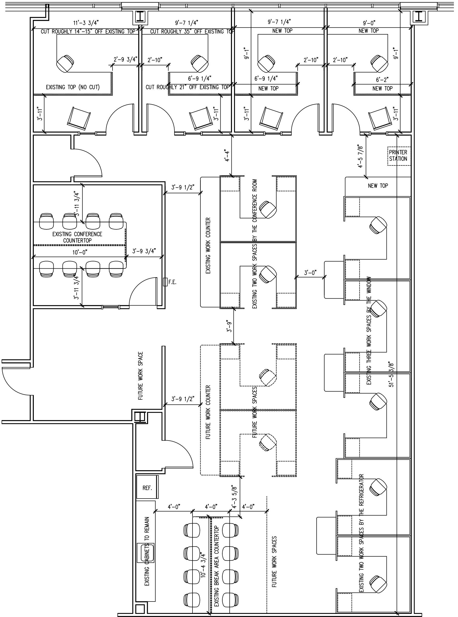
BLUE FROG DESIGN OFFICE – SUITE 340 FLOOR PLAN / CABINET PLAN
