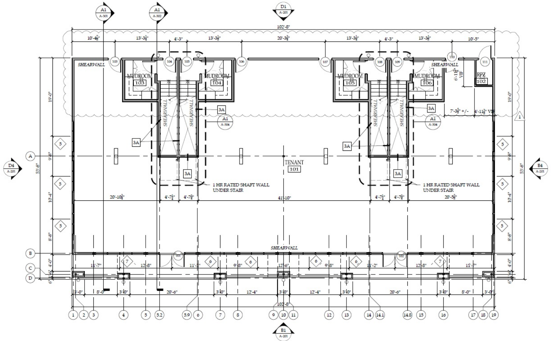
A1 FIRST FLOOR PLAN 1/8"=1'-0"
