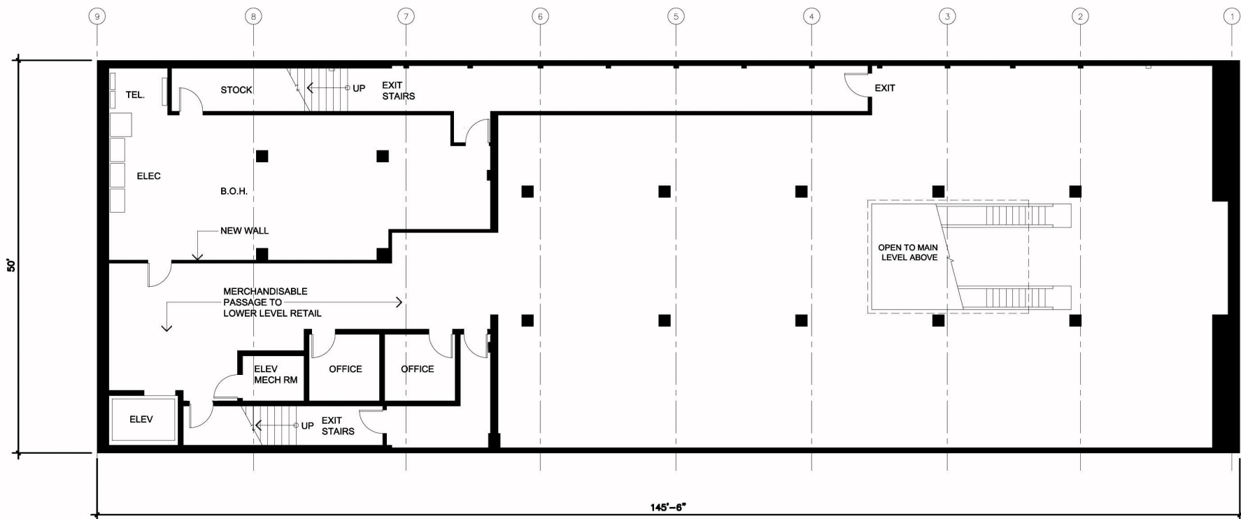
LOWER LEVEL PLAN - DESIGN OPTION A 7275 sf
