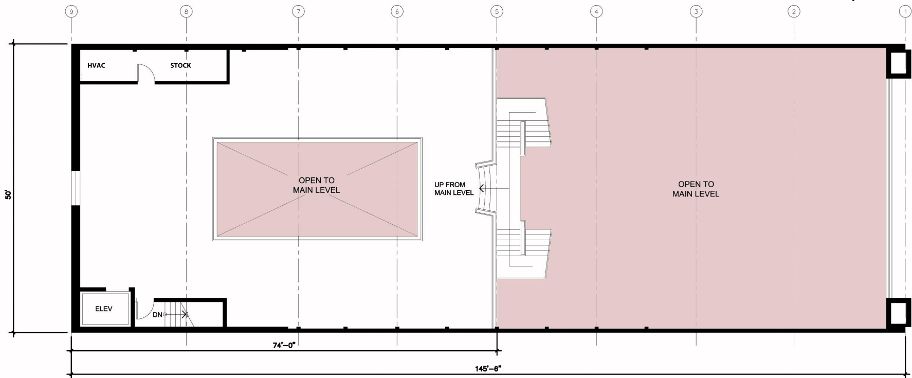
UPPER LEVEL PLAN - DESIGN OPTION A 3700 sf
