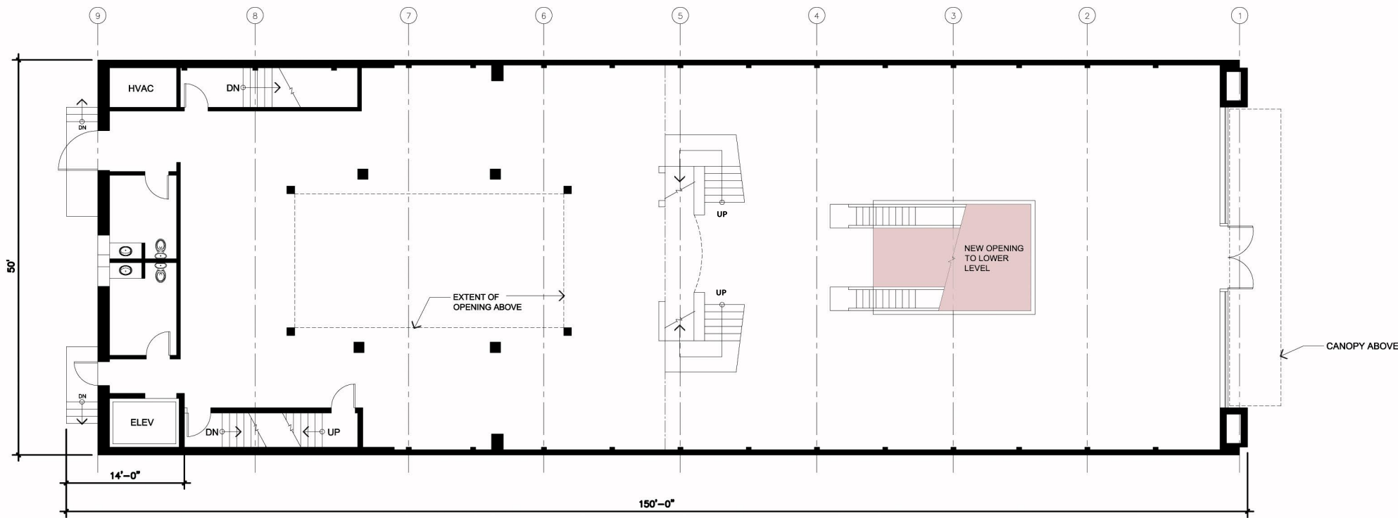
MAIN LEVEL PLAN - DESIGN OPTION A 7500 sf
