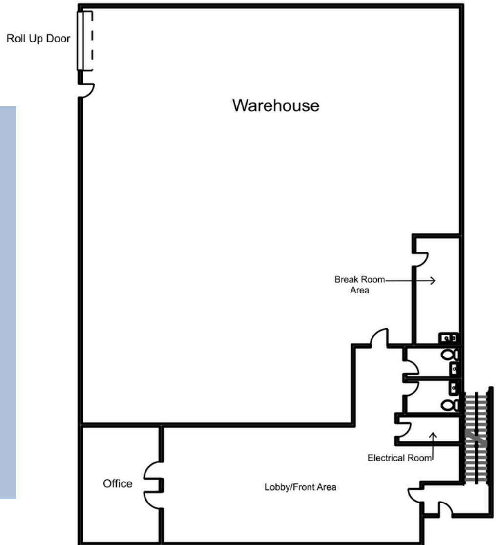
1st Floor
