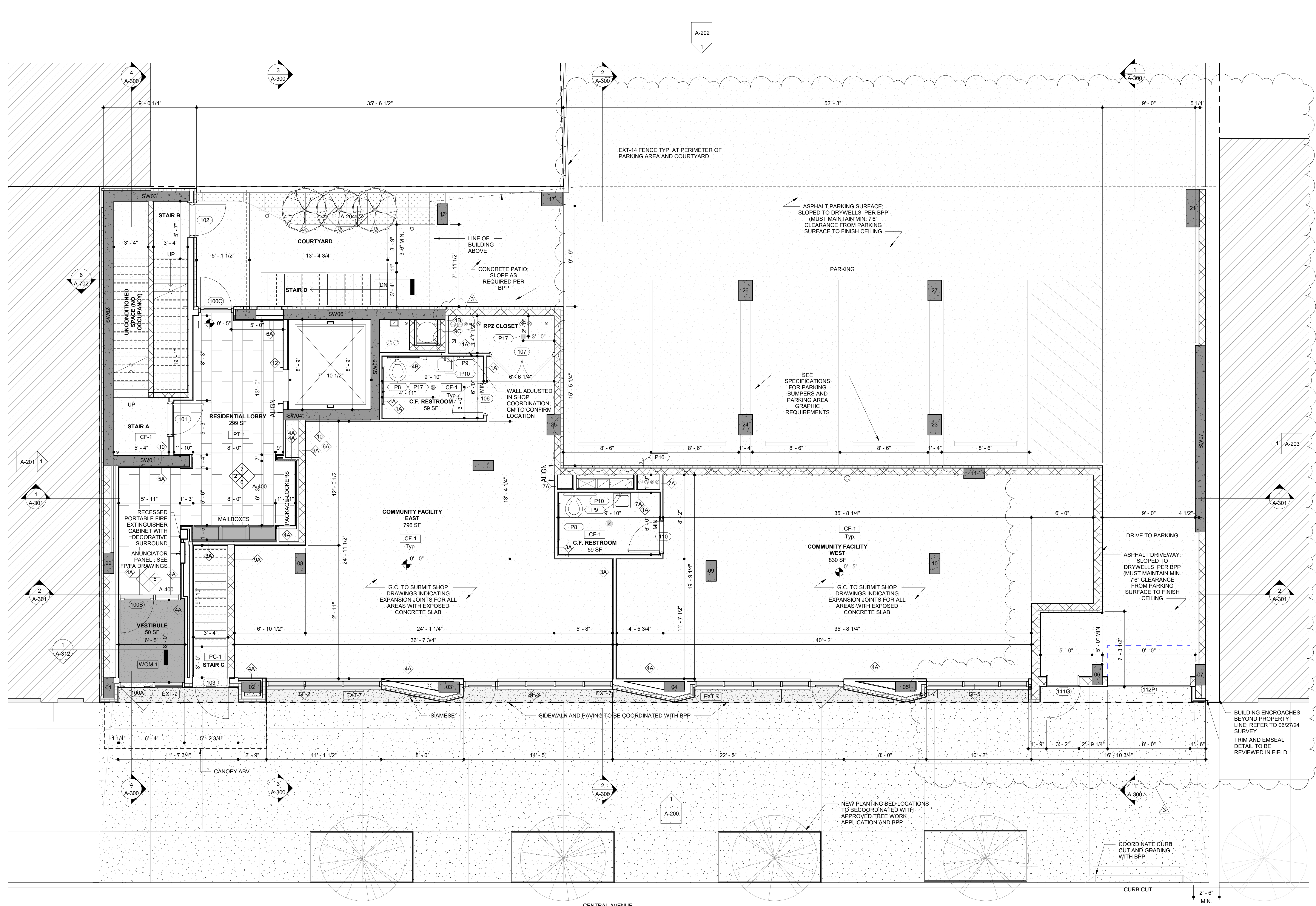
1 1st Floor Construction Plan 1/4" = 1'-0"
