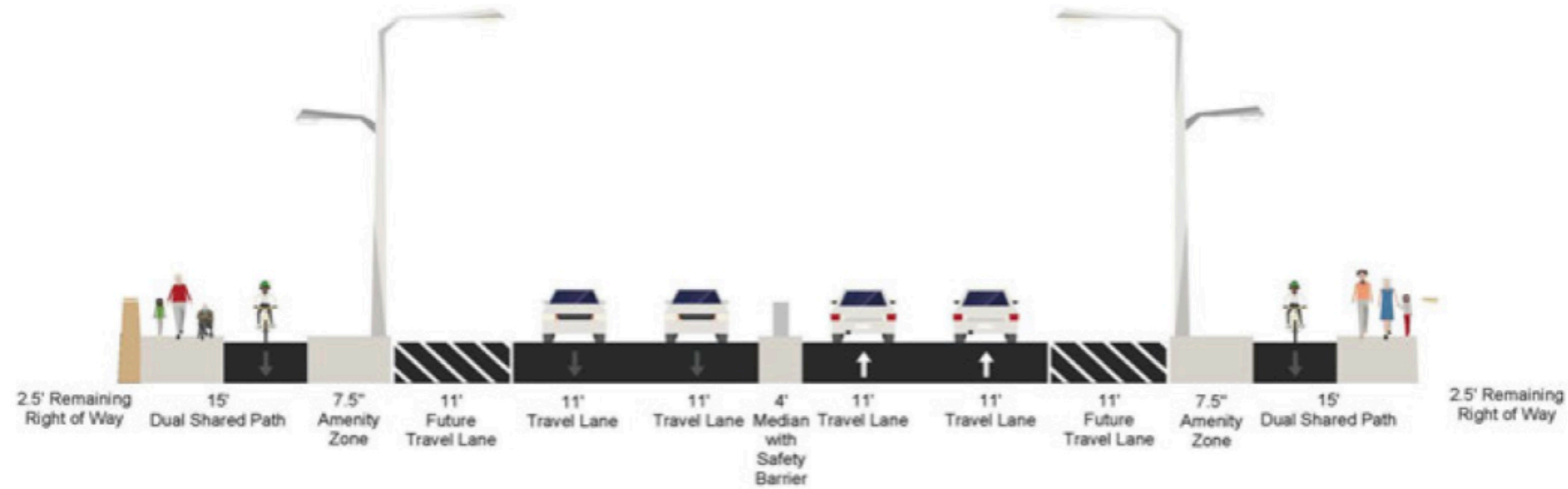
Figure 1: Bonds Ranch Road Proposed Roadway Typical Section
