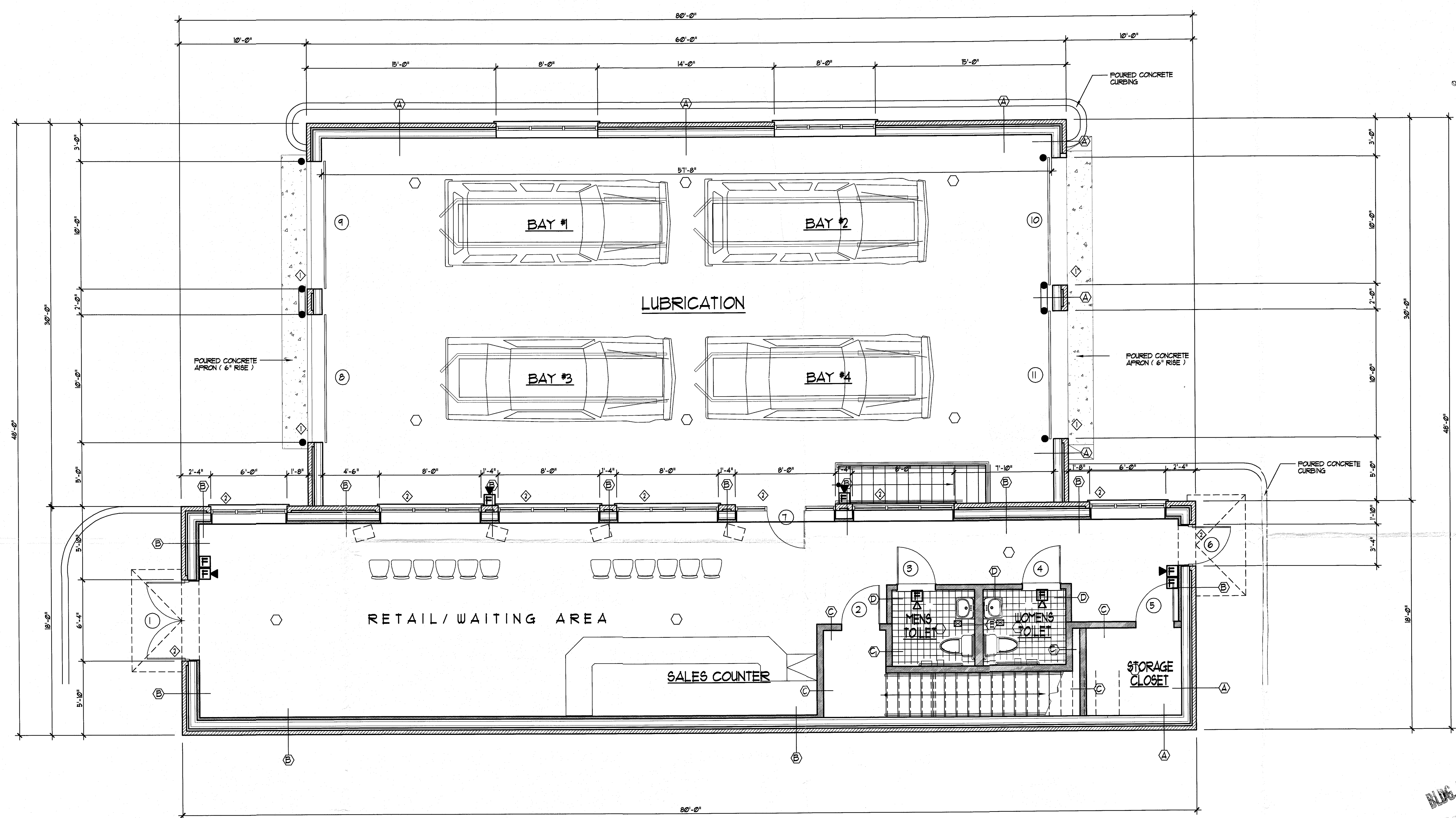
FLOOR PLAN
