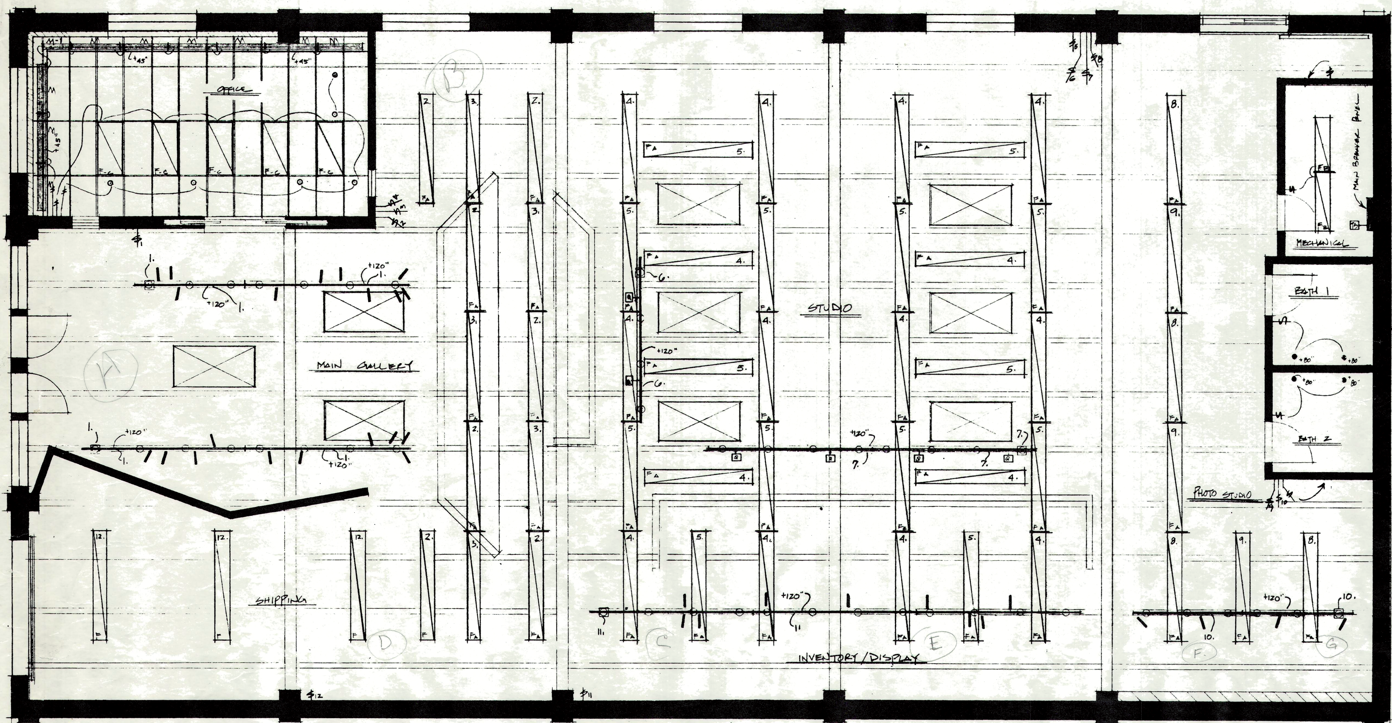
REFLECTED CEILING @ STUDIO
