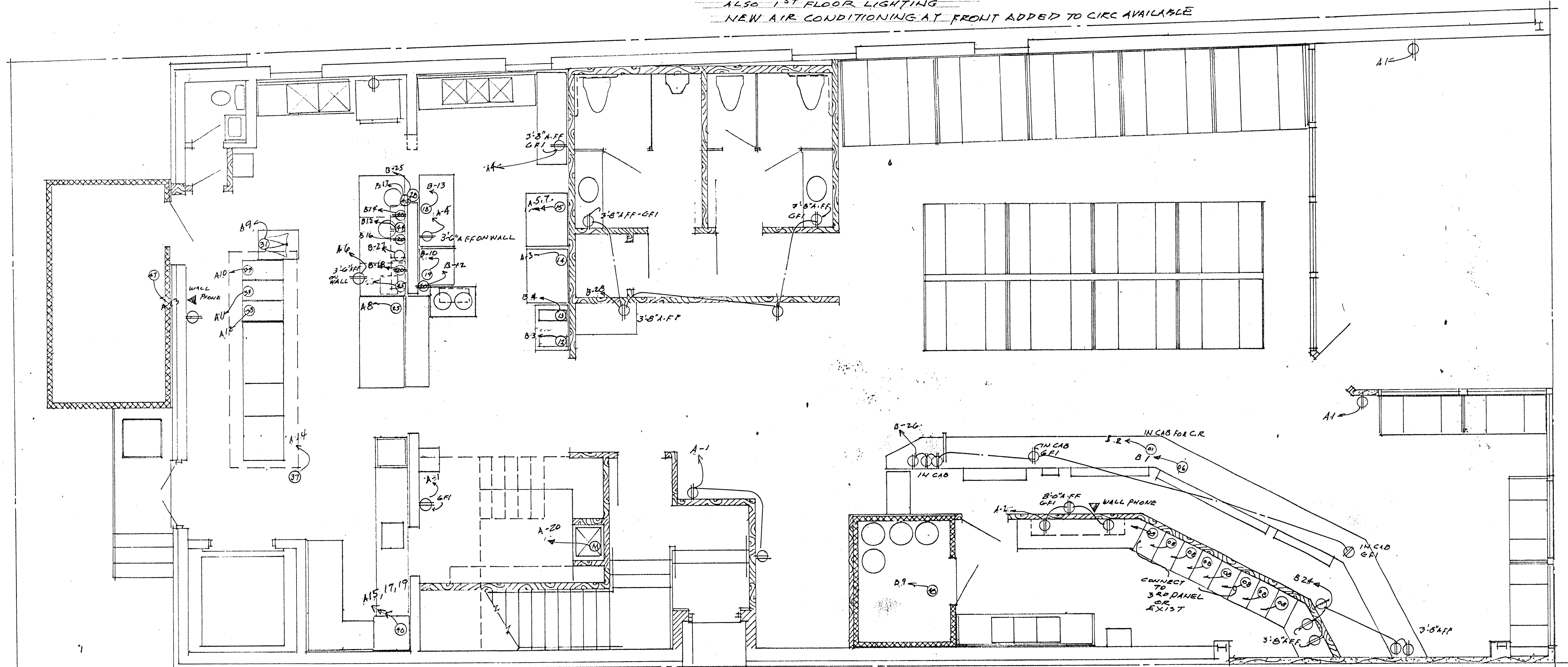
ELECTRICAL OUTLET PLAN FLOOR PLAN SCALE 1/4" = 1'-0"
