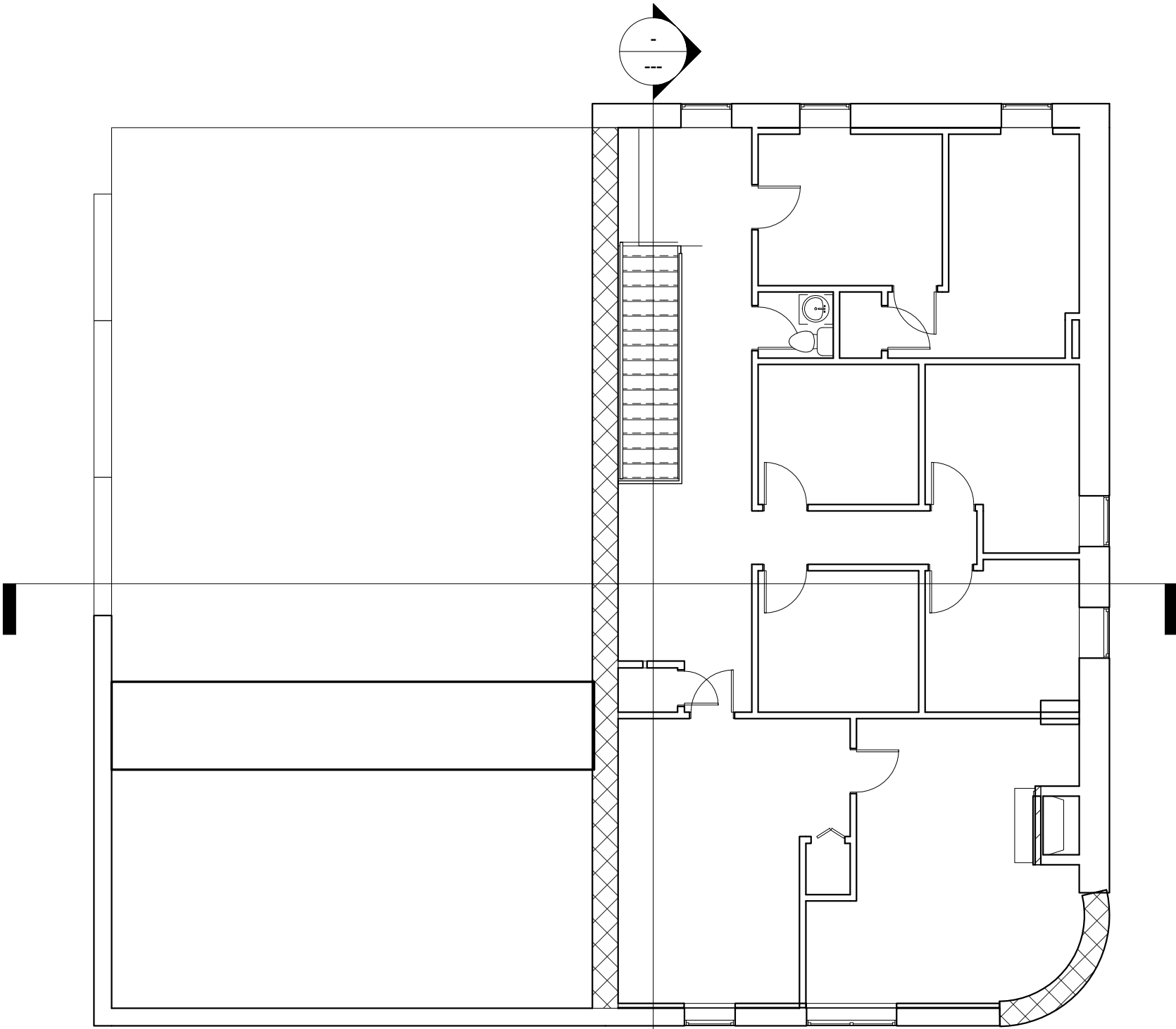
644 West Main, Third Floor Level
