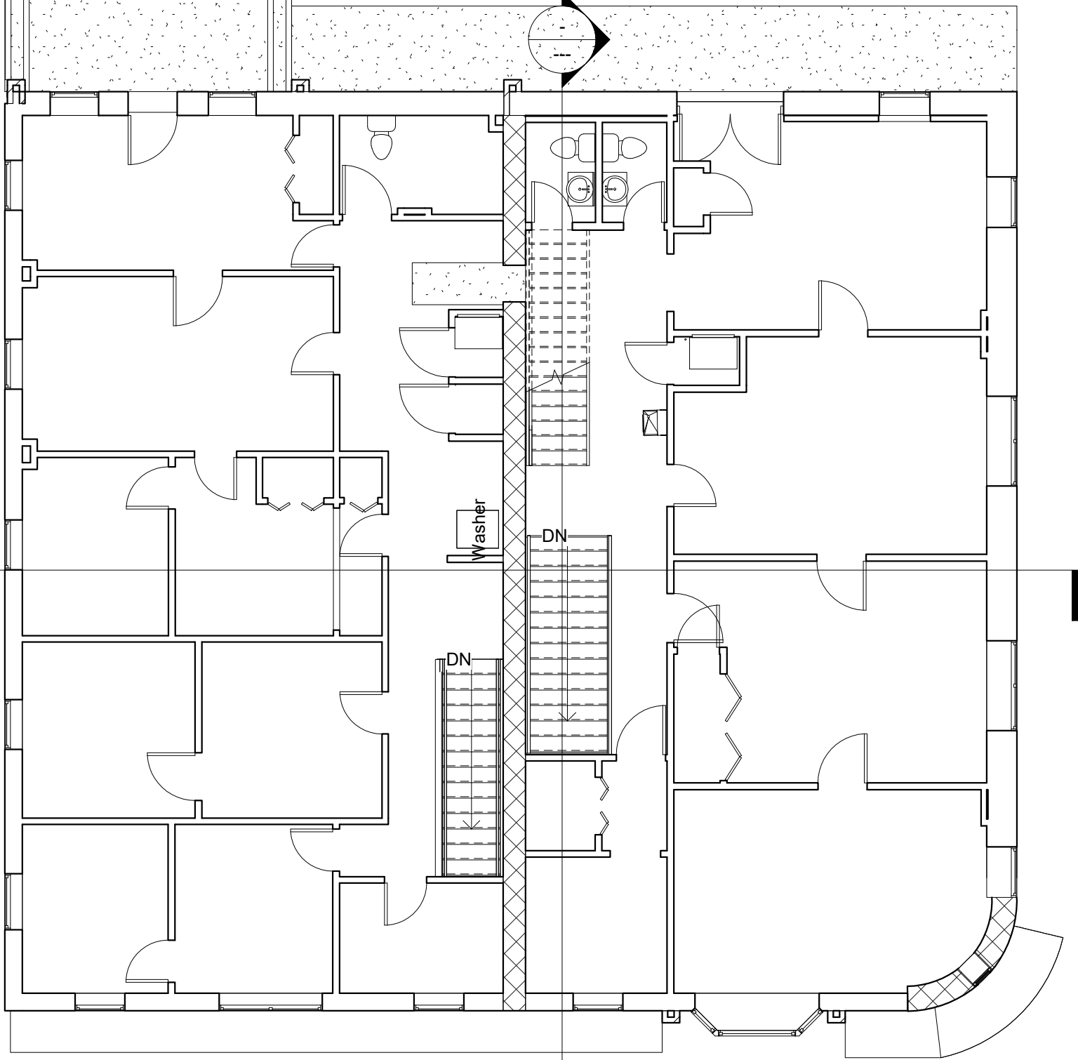
642 West Main, Rear Parking Area Level
