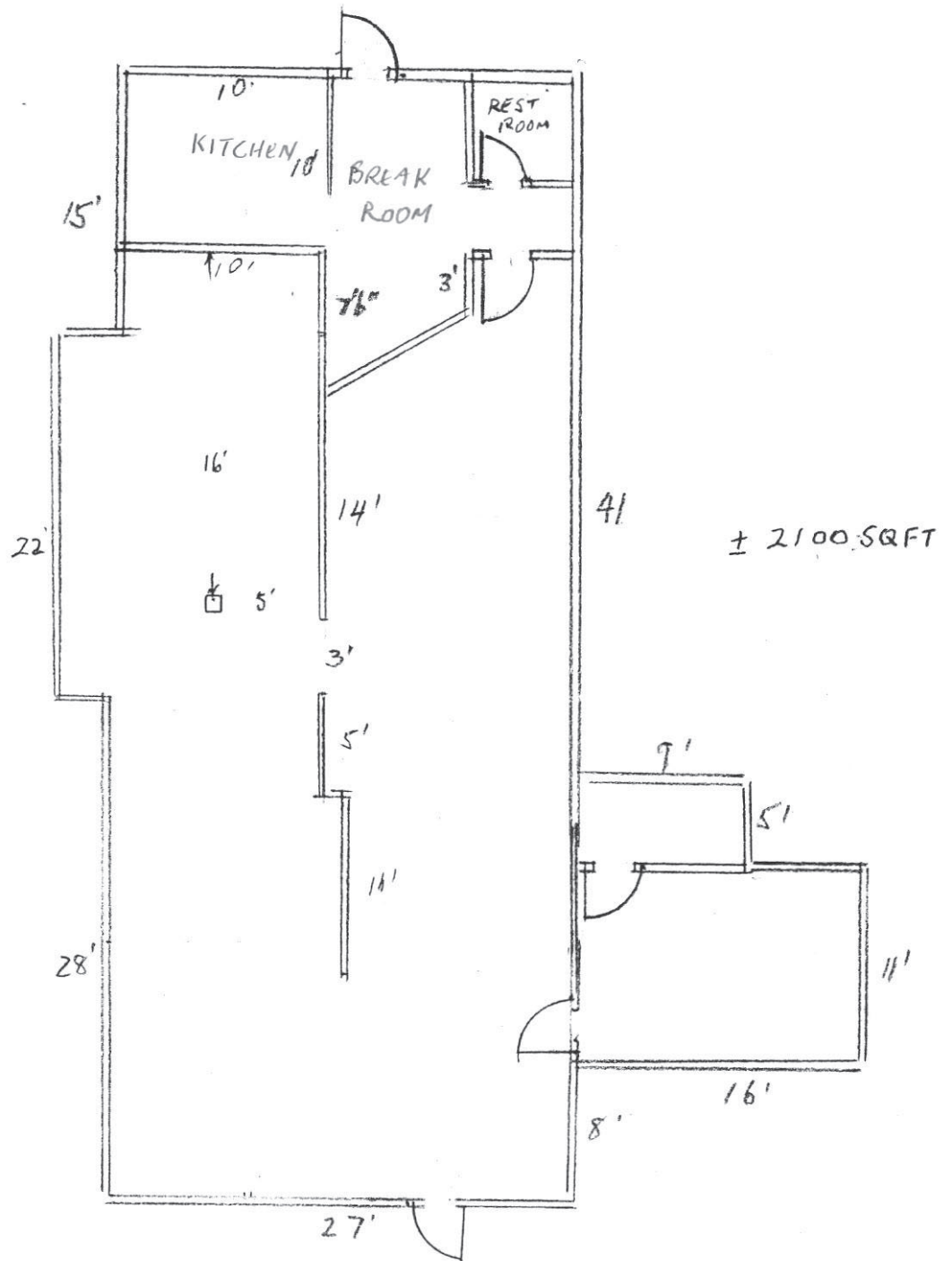
FLOOR PLAN SUITE 4-7 2033 AIRLINE ROAD CORPUS CHRISTI TX 78412
