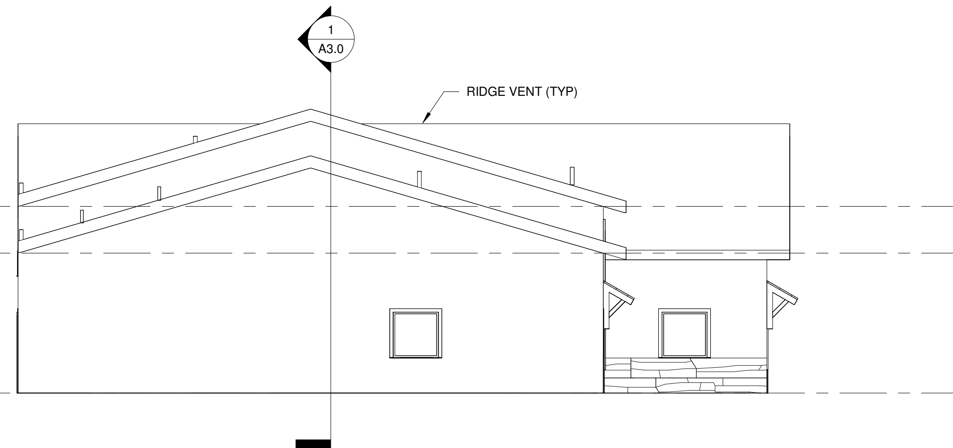
Right Elevation 1/8" = 1'-0"
