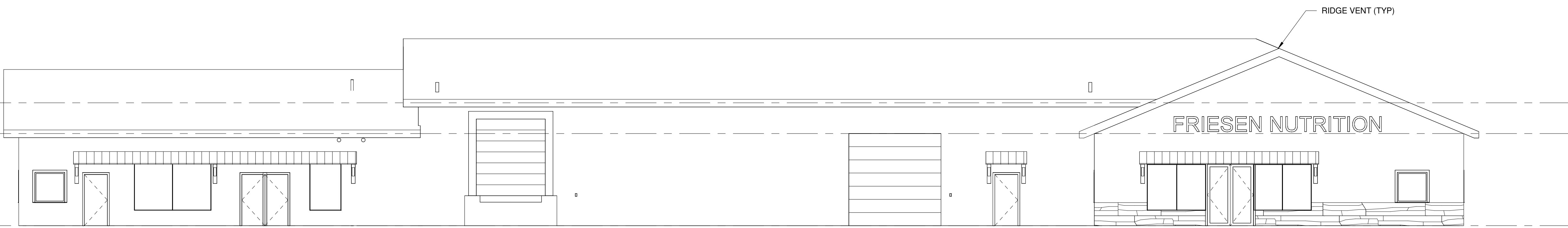
Front Elevation 1/8" = 1'-0"
