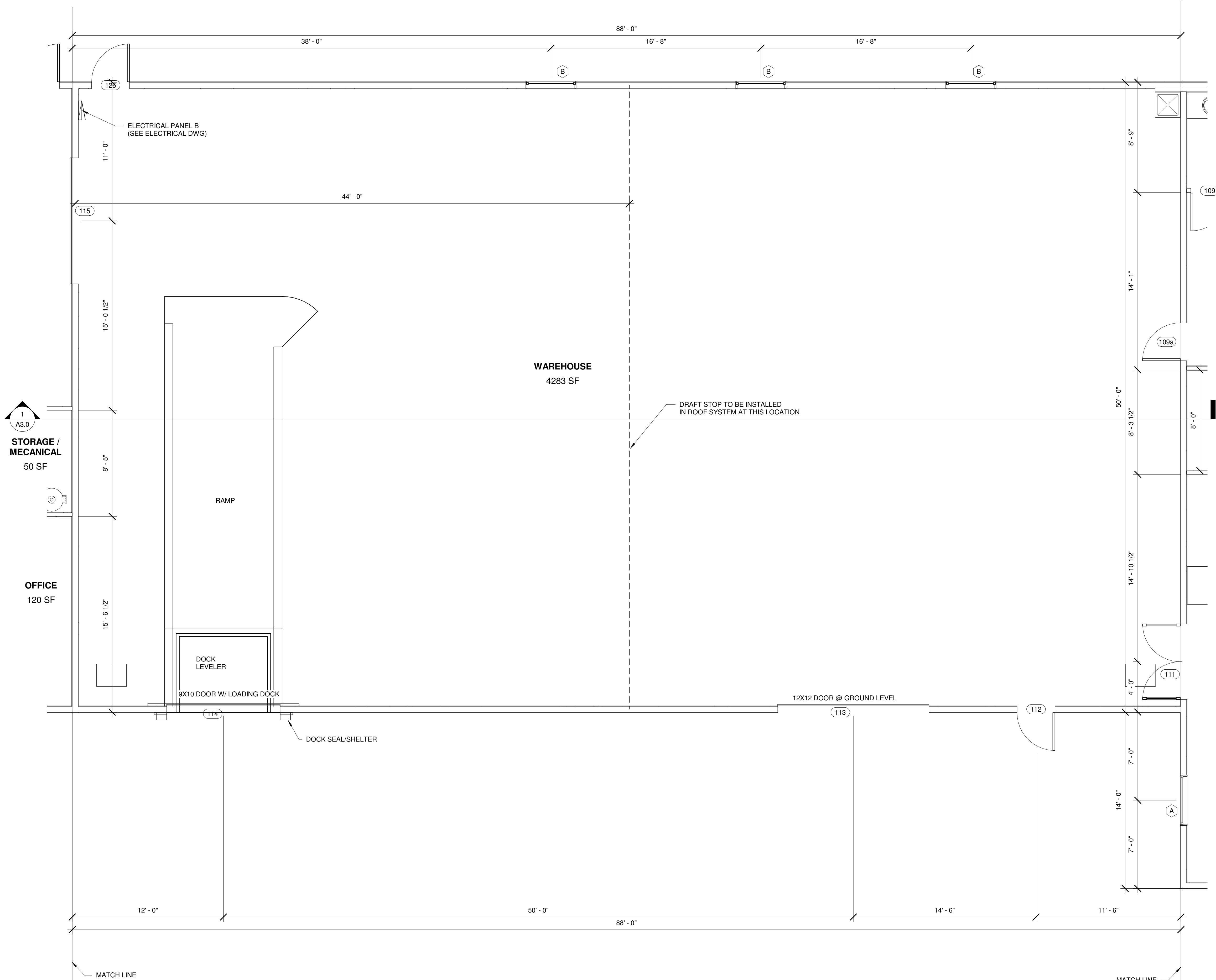
FLOOR PLAN - WAREHOUSE 1/4" = 1'-0"
