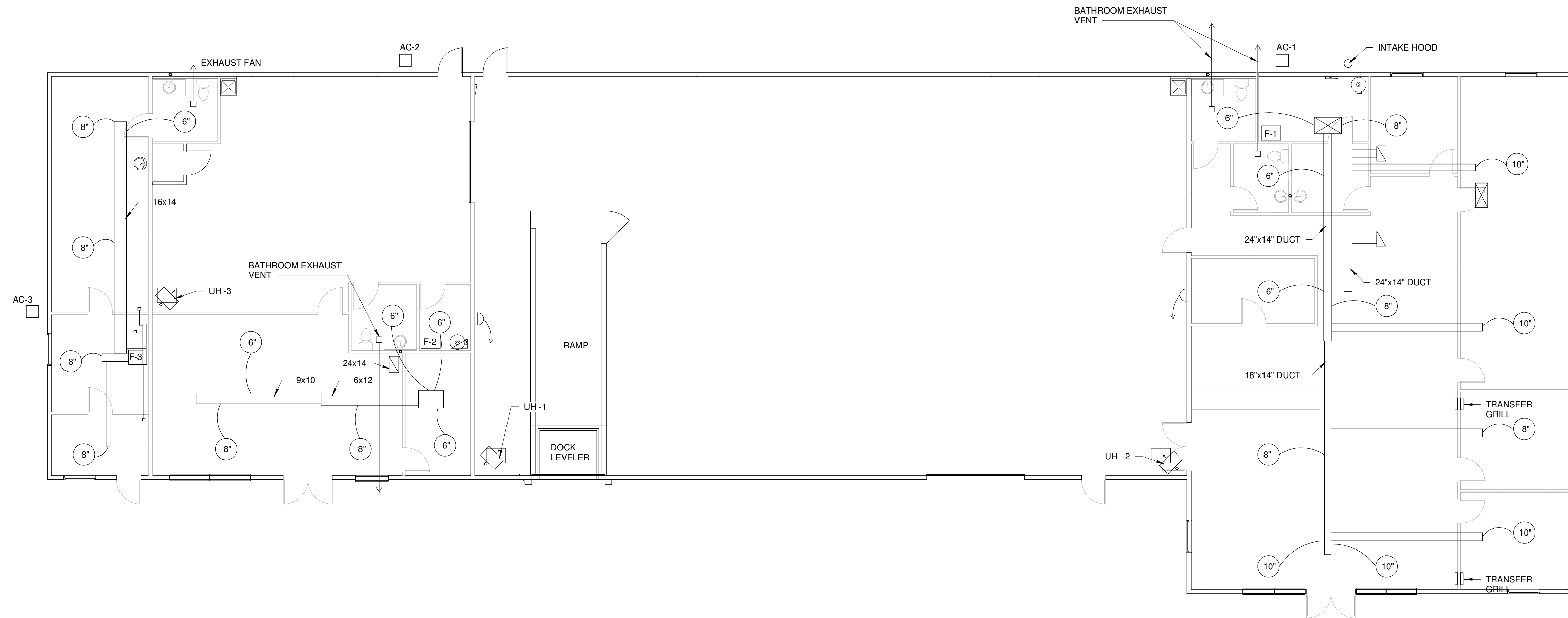
MECHANICAL PLAN 1/8" = 1'-0"
