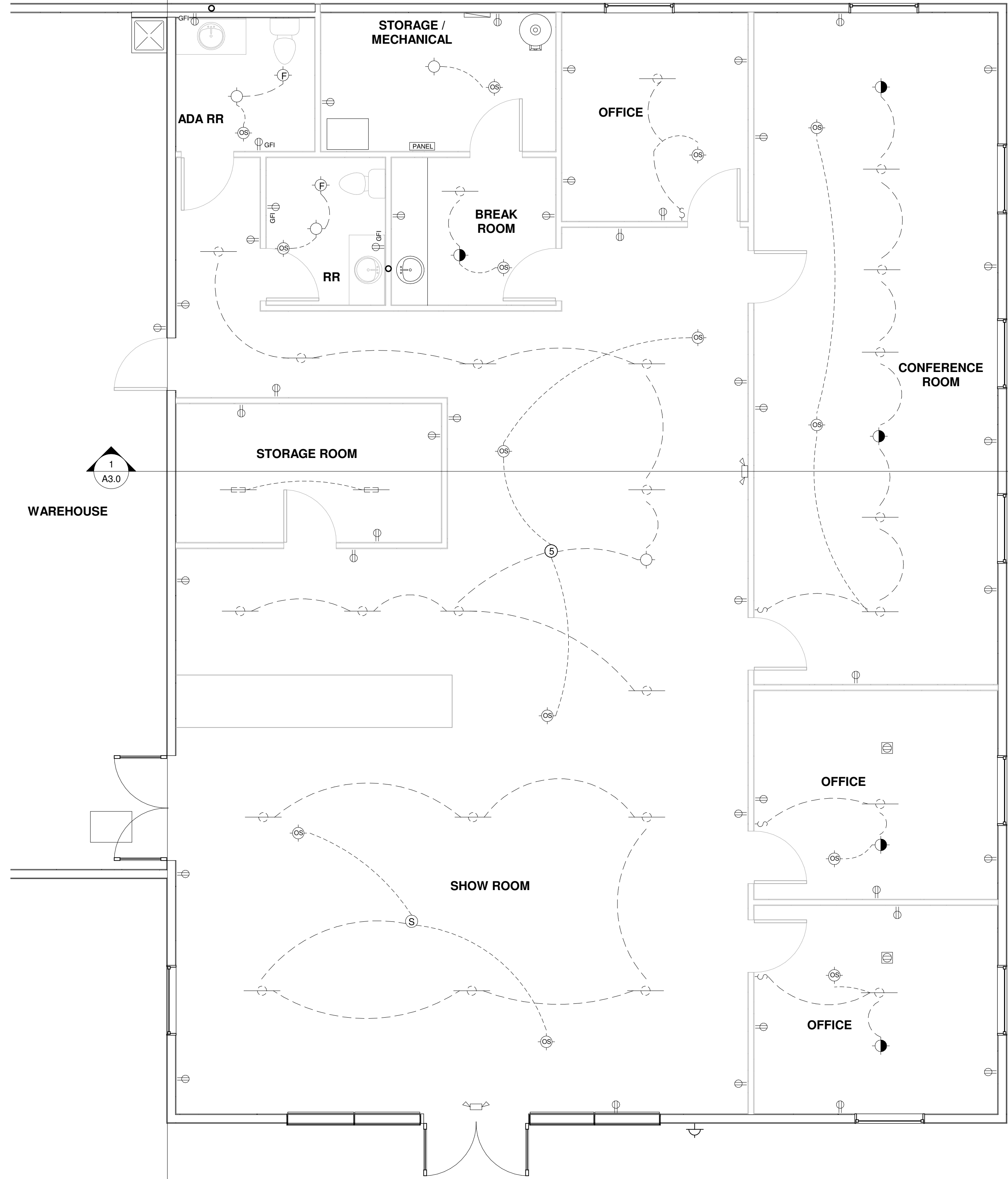
ELECTRICAL - SHOWROOM 1/4" = 1'-0"
