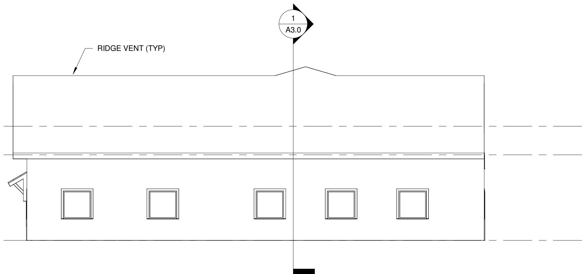
Left Elevation 1/8" = 1'-0"
