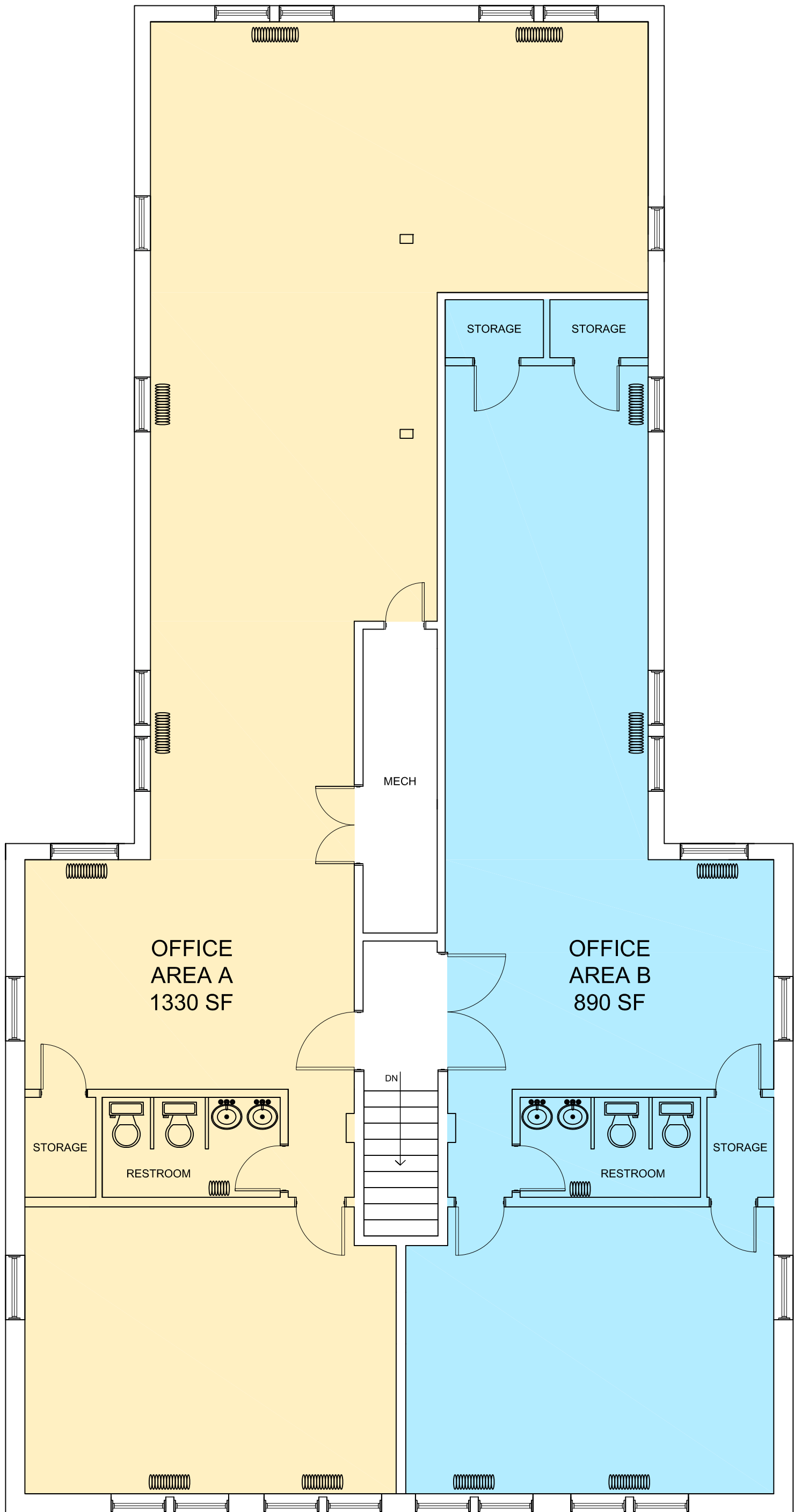
2010 RHODE ISLAND AVE NE - SECOND FLOOR SCALE: 3/16" = 1'-0"
