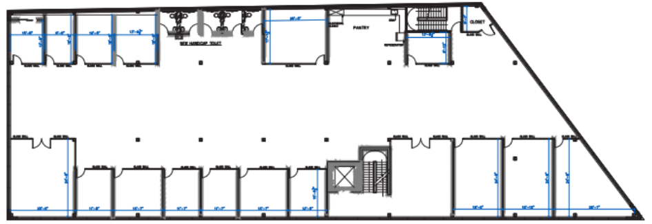
2nd FLOOR PLAN SCALE: 1/8" = 1'-0"
