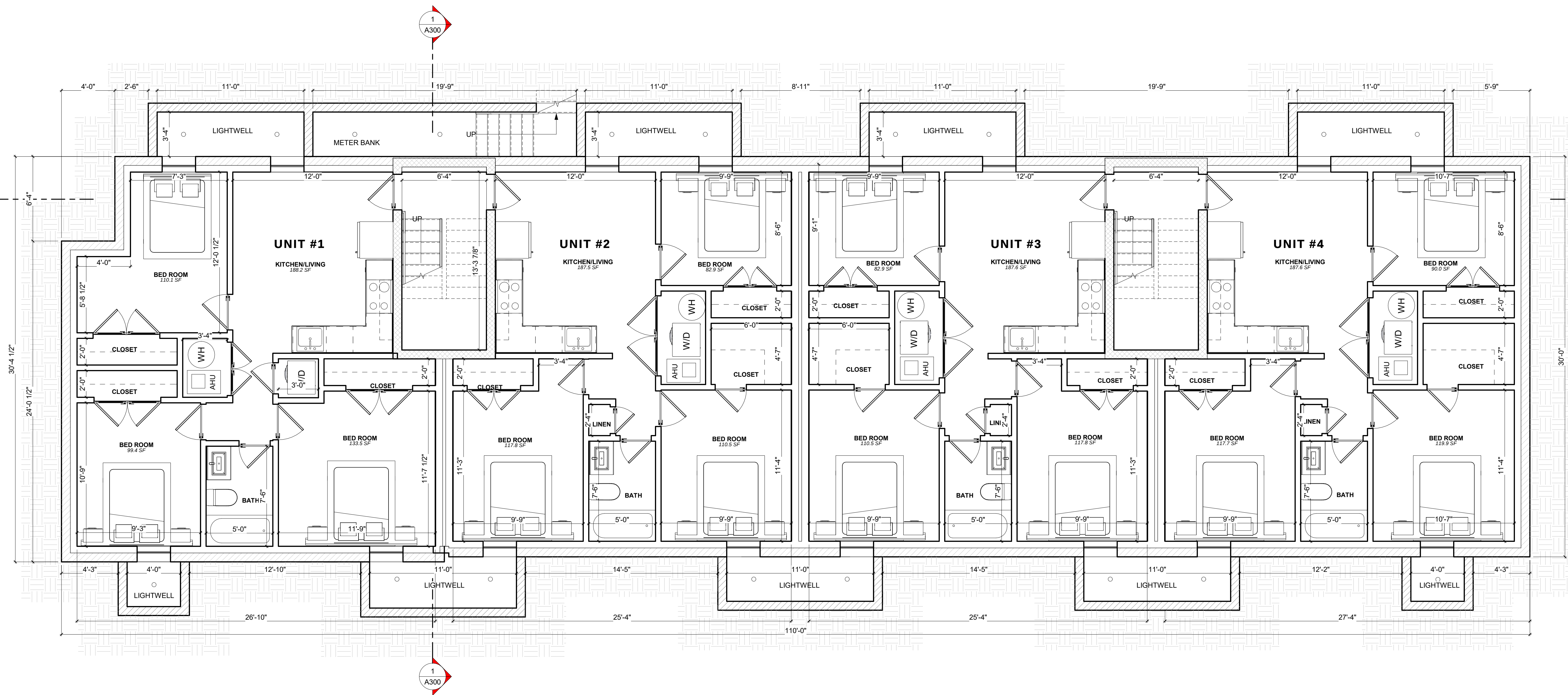
1 Cellar Level 1/4" = 1'-0"
