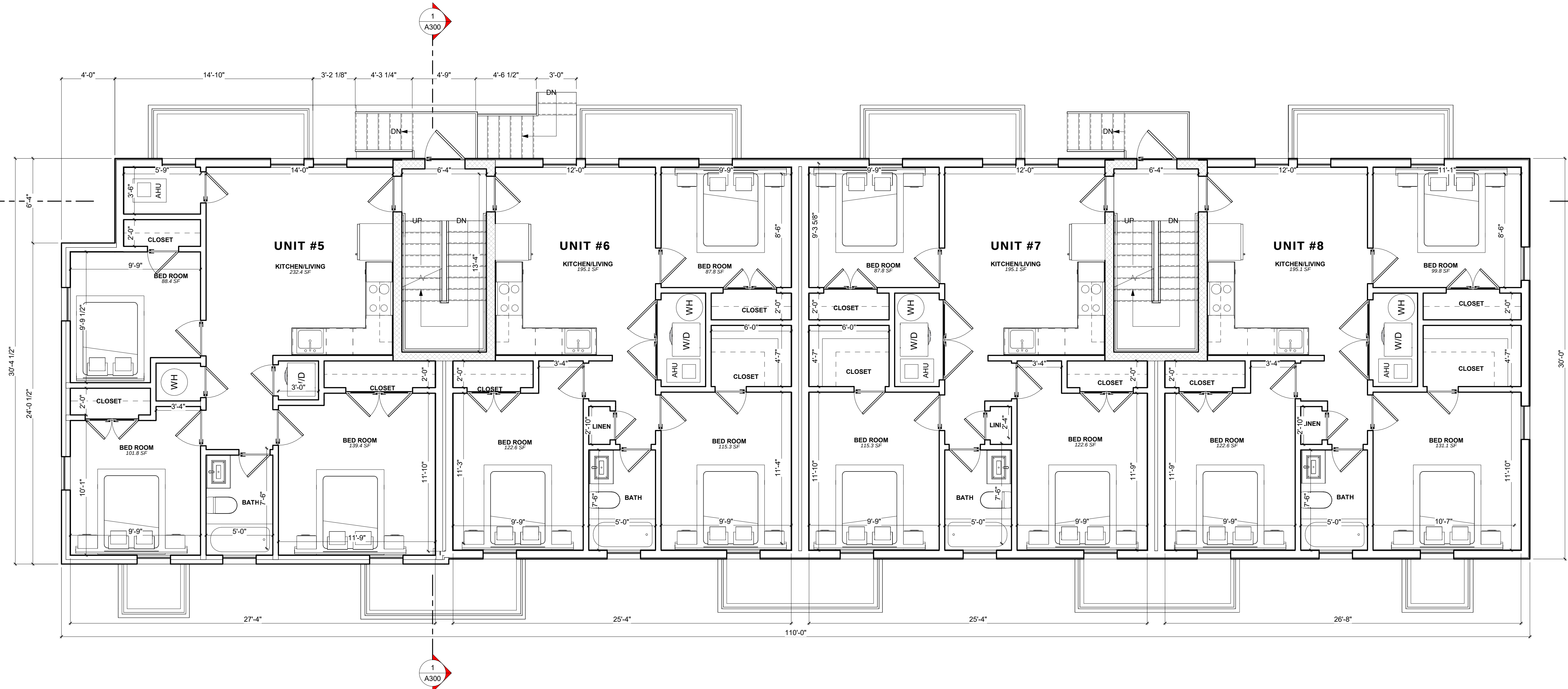
2 First Floor 1/4" = 1'-0"
