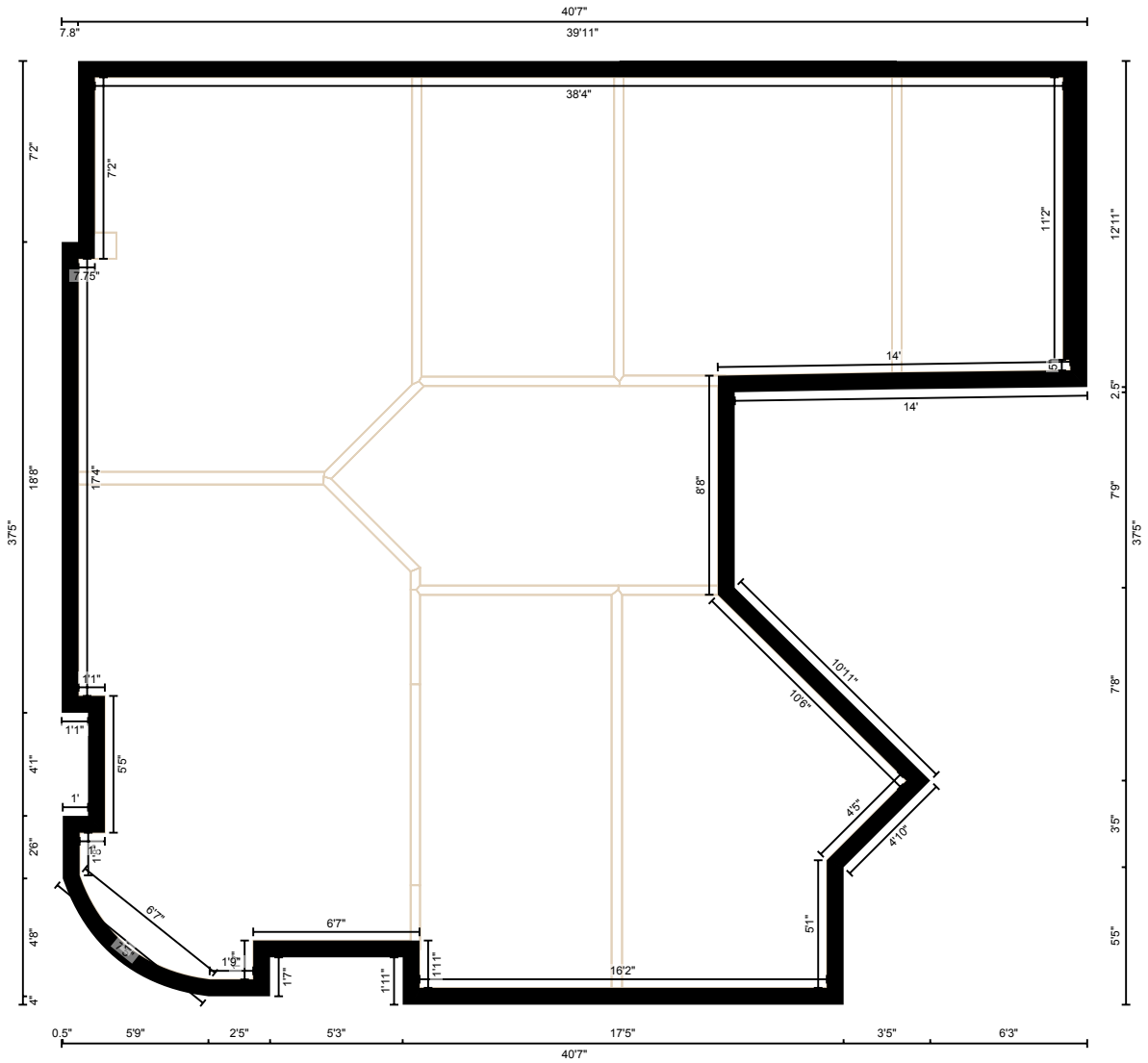
Measurement Diagram for: Main Floor
