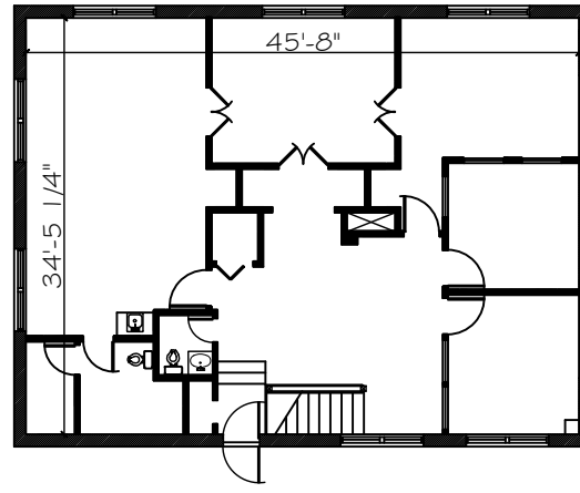
THIRD FLOOR PLAN SCALE: 1/4" = 1'-0"
