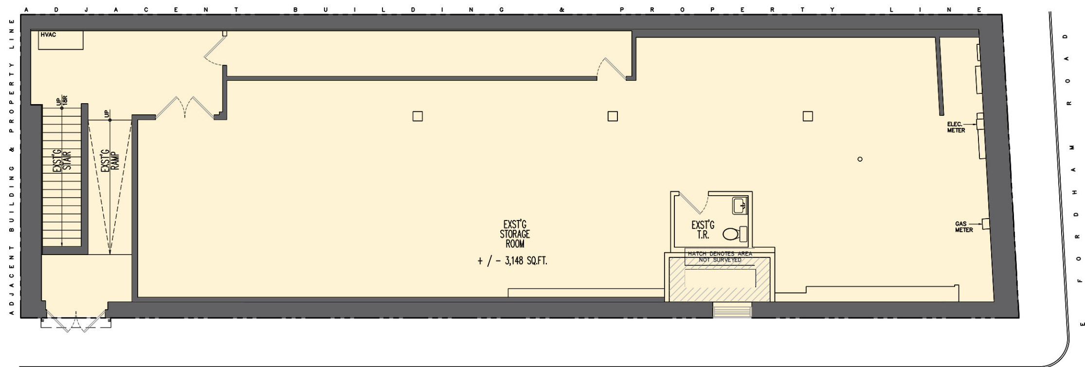
② EXISTING CELLAR FLOOR PLAN
