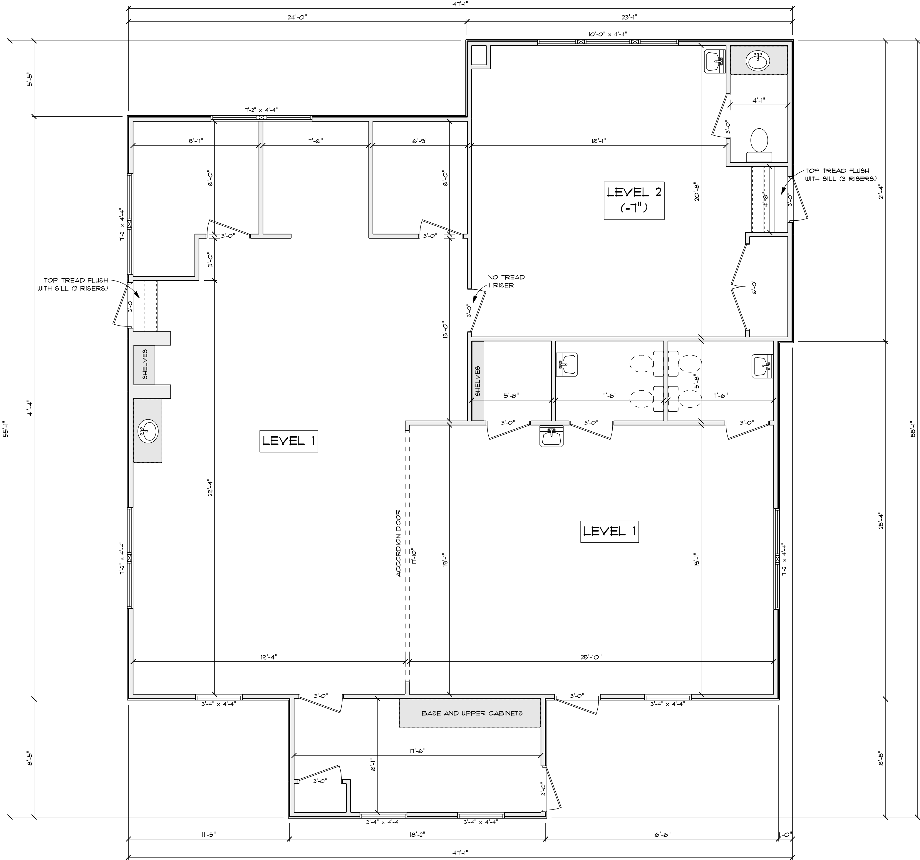
MAIN LEVEL EXISTING SCALE: 1/4" = 1'-0"
