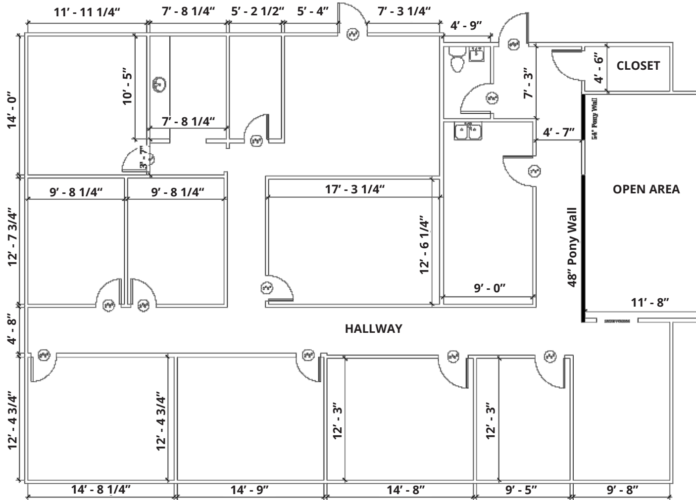
A-1 FLOORPLAN 1 3/8" = 1'-0"
