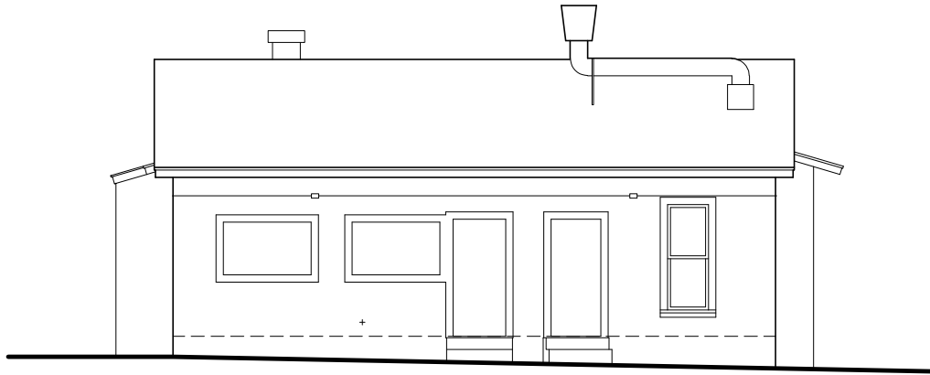
REAR ELEVATION
