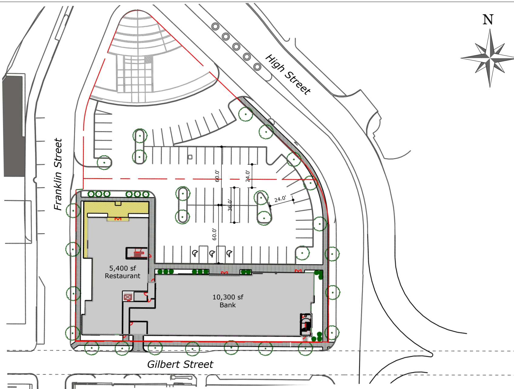
SITE LAYOUT
