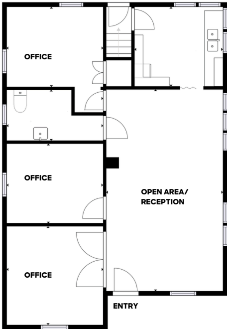
MAIN FLOOR
