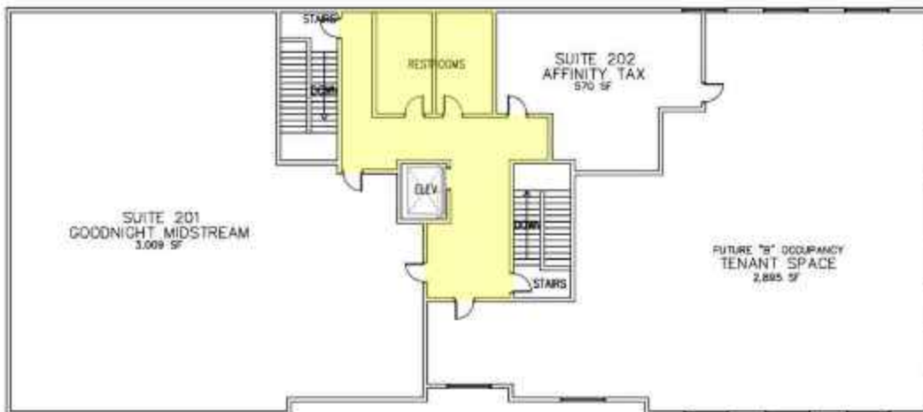
SECOND FLOOR PLAN 1/8" = 1'-0"
