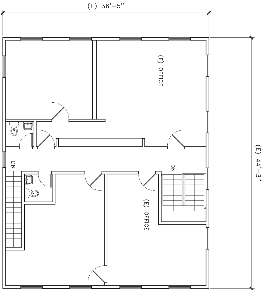
(E) SECOND FLOOR PLAN
