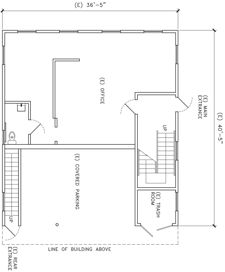
(E) GROUND FLOOR PLAN
