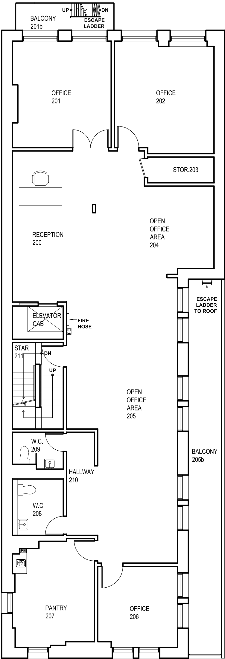
2ND FLOOR scale: 1/8"=1'-0"
