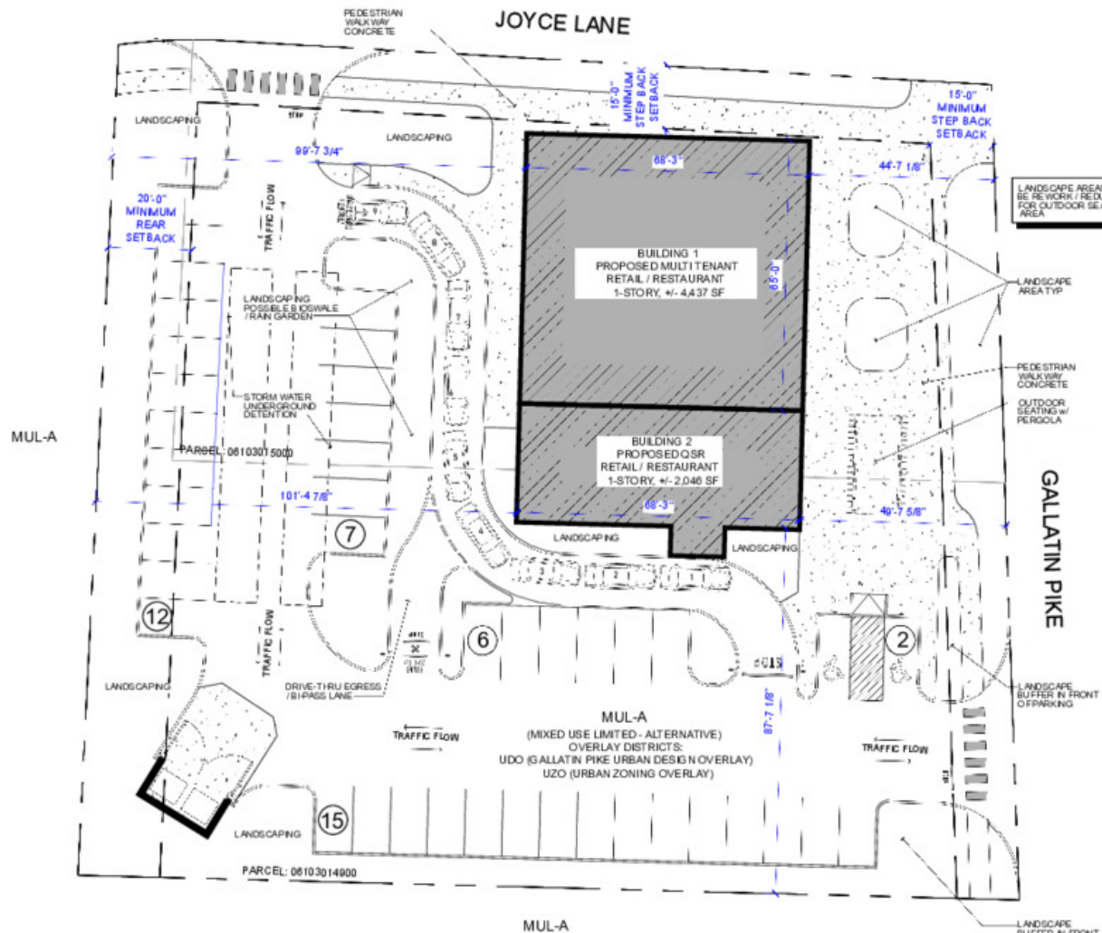
OPTION 3 R1 SCHEMATIC SITE PLAN SCALE: 1" = 20'-0" 1 AS.101
