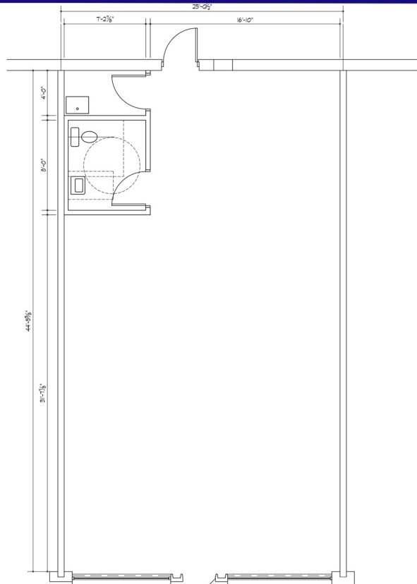
EXISTING FLOOR PLAN 15463 CLAYTON RD BALLWIN, MISSOURI
