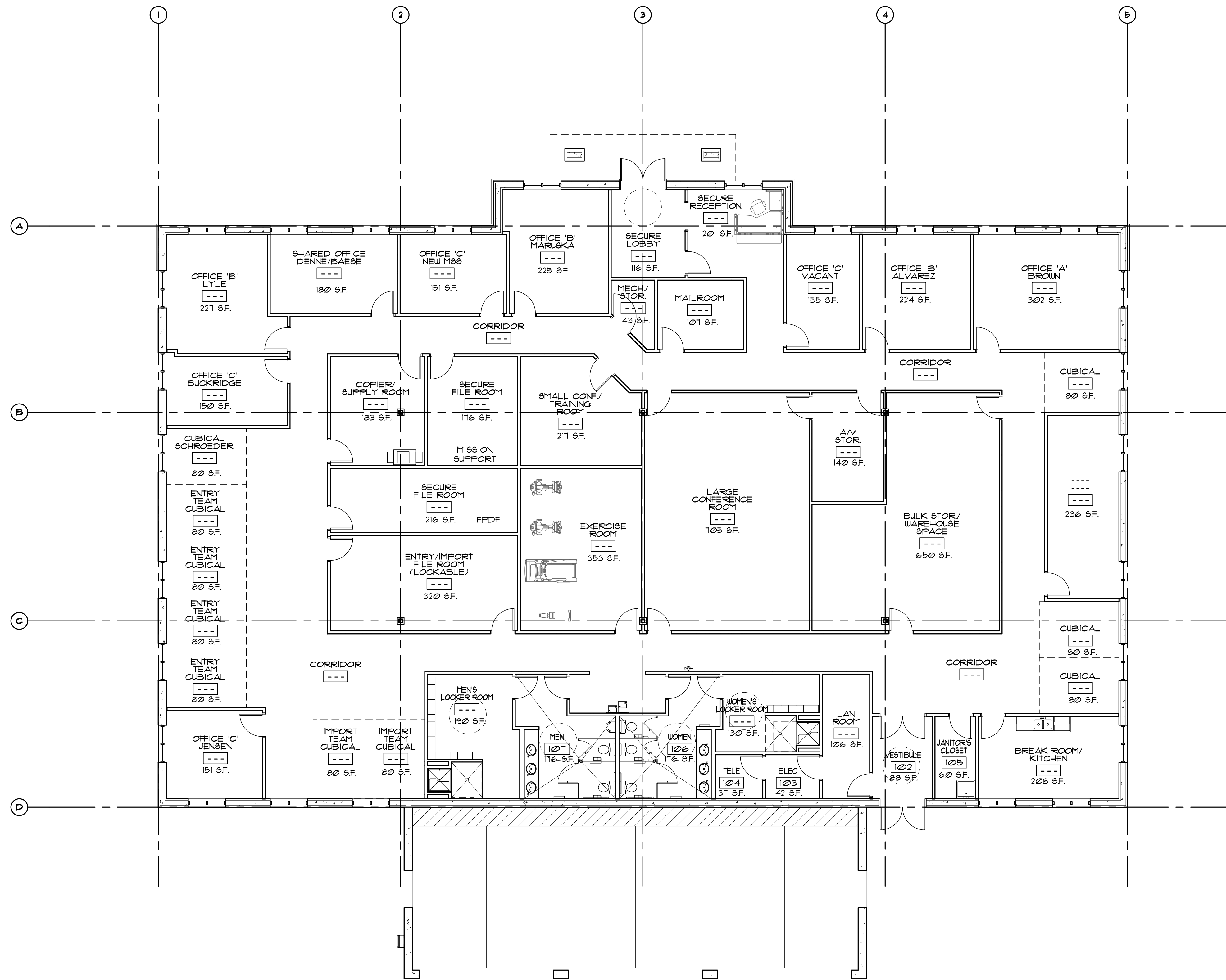
1 TENANT IMPROVEMENTS SPACE PLAN 1/8" = 1'-0"
