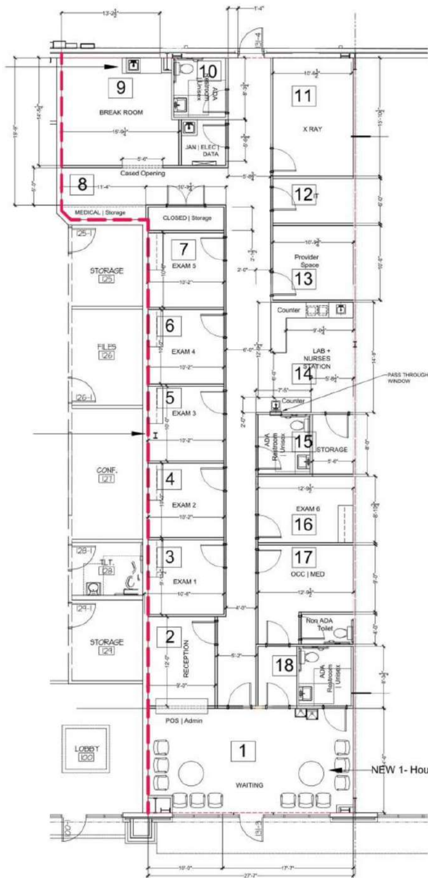
1 FLOOR PLAN A2 Work Area Limits Schematic 1/16" @ 24x36 NOTE | Dimensions provided are approximate
