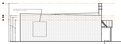
Proposed Left Side Elevation
