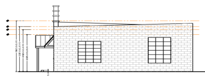
Proposed Right Side Elevation
