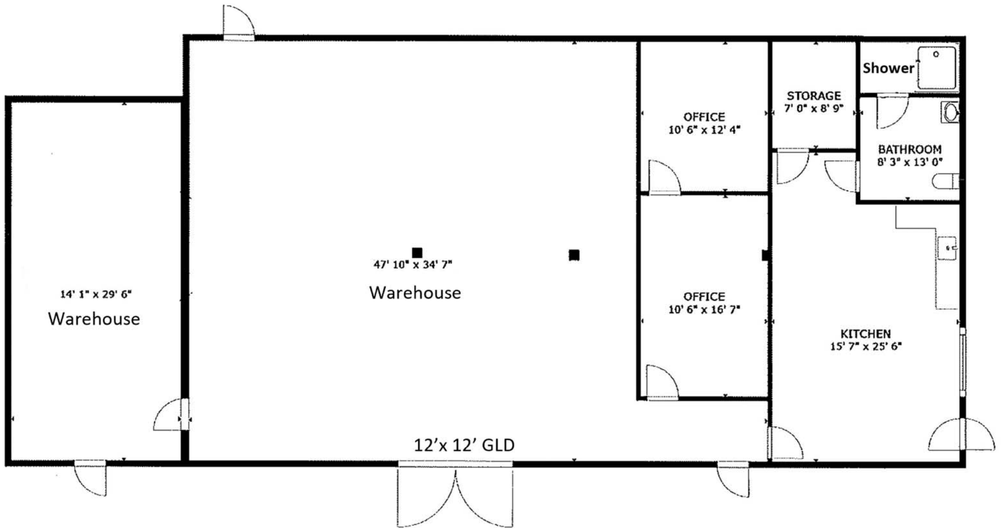
FLOOR PLAN
