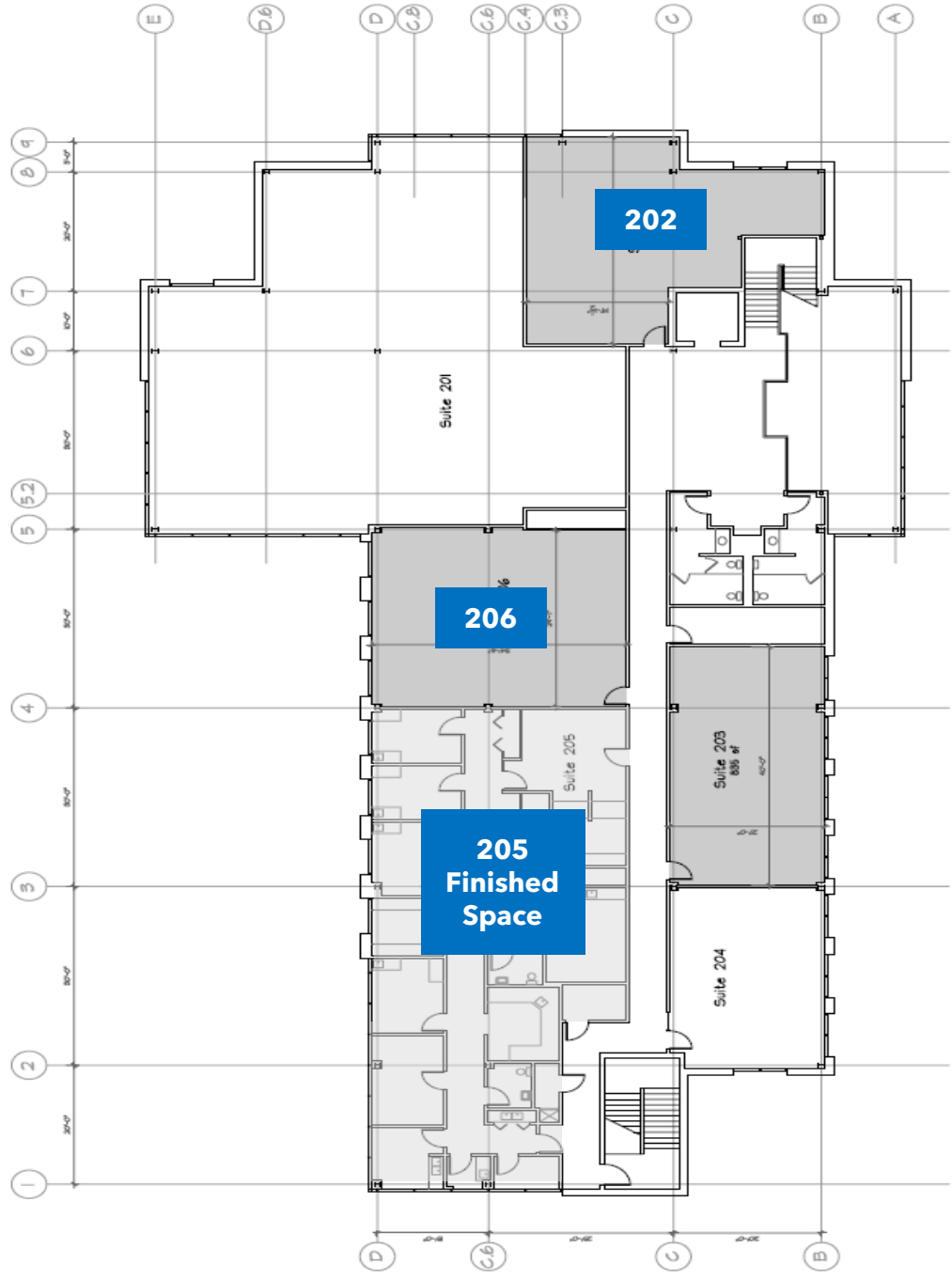
EXISTING SECOND FLOOR PLAN Scale (1/8" = 1'-0")
