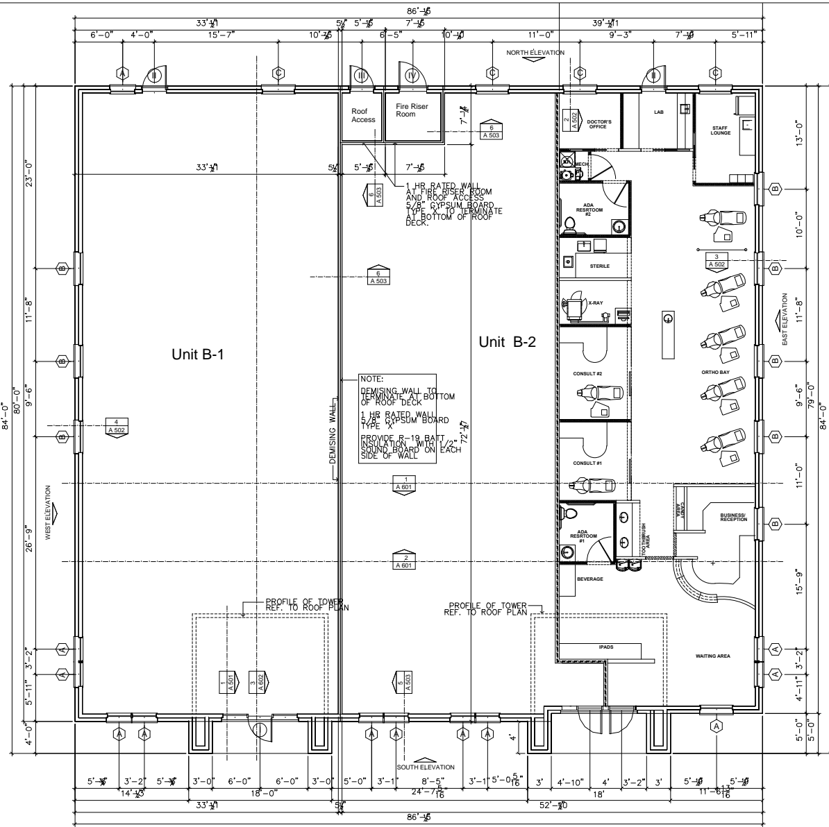
1 Floor Plan SCALE: 3/16" = 1'-0" UNIT B-1 2666SQ.FT. UNIT B-2 4126SQ.FT. TOTAL 6792SQ.FT. RISER RM 33FT. ROOF ACCESS 39FT. GRAND TOTAL 6888SQ.FT.
